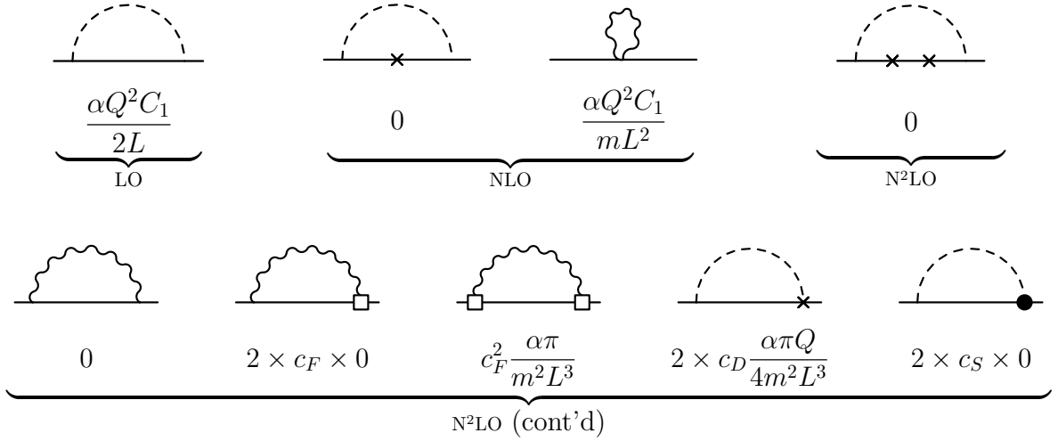
Figure 1: NREFT self-energy diagrams which contribute to finite-volume effects on the mass of a spin-1/2 particle, up to order 1/L^3 . Their contributions were taken into account in [14]. The solid line corresponds to the fermion propagator; the dashed line to the temporal photon propagator; the wavy line to the transverse photon propagator; the cross to a kinetic term insertion; the simple vertices with these lines, to the fermion-temporal-photon interaction; to the fermion-transverse-photon interaction; to the fermion-to-two-transverse-photons interaction; the square vertex to the Fermi interaction; the crossed vertex to the Darwin interaction; the dot vertex to the spin-orbit interaction. Under each diagram we indicate its contribution to the finite-volume correction on the fermion mass. Calculations are performed in Coulomb gauge. An explicit factor of 2 appears in the single Fermi, Darwin and spin-orbit vertex terms. This indicates that to each of the three diagrams shown corresponds one in which the vertices are switched. These new diagrams give the same contributions as the original diagrams. The sum of all the contributions shown in the figure yields the result in Eq. (2).
