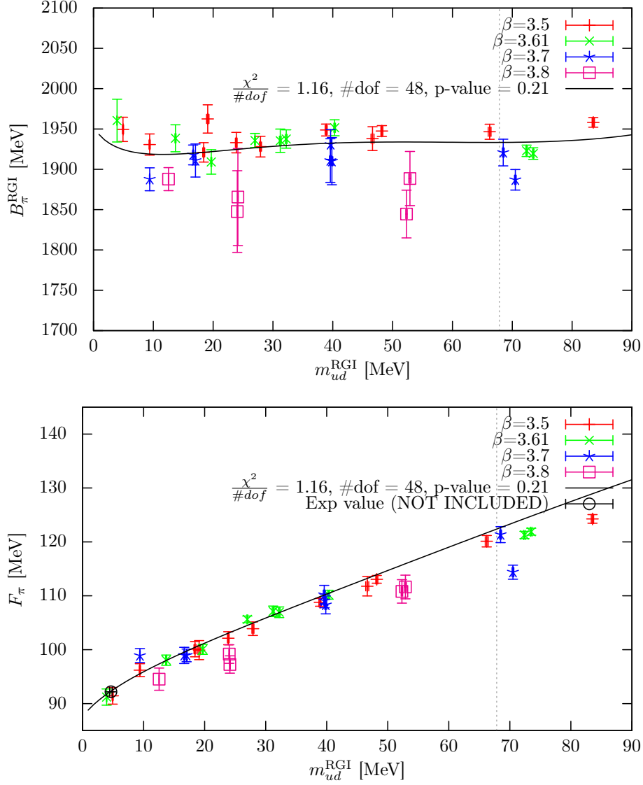
Figure 3: Typical NNLO SU(2) \chi PT fit (curves) of our lattice results (points with error bars) for B_{\pi} and F_{\pi} as functions of m_{ud} , in the x -expansion. Only points with M_{\pi} \leq M_{\pi}^{\text{max}} = 500 MeV (i.e. m_{ud}^{\text{max}} \lesssim 65 MeV) are included in the fits, i.e. those left of the dashed vertical line. The description is the same as in Fig. 1, except that the functional forms used are those of (14) with B_{\pi}^{x-NLO} and F_{\pi}^{x-NLO} replaced by B_{\pi}^{x-NNLO} and F_{\pi}^{x-NNLO} , respectively.
