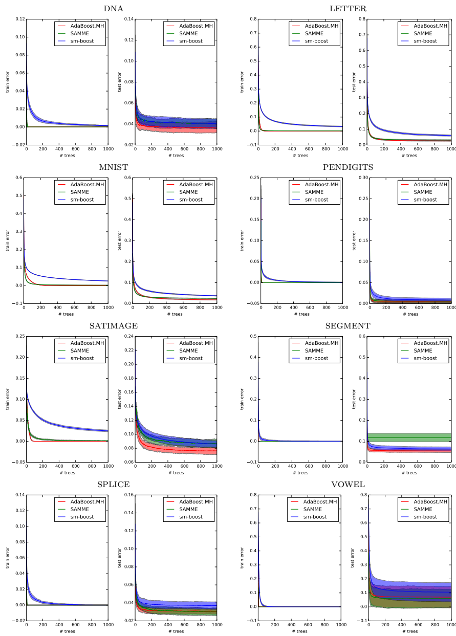
Fig. 5 Train and test error curves for the considered data sets.
