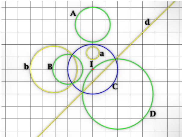
Figure 1: Different effects of inversion, according to the respective positions of the circles.
