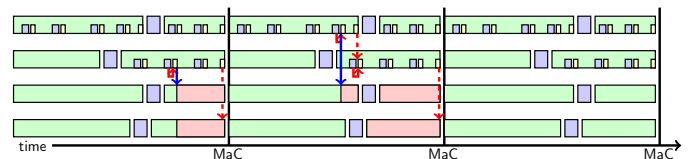
Figure 9. Example of internal deadline adaptation when LRM inside critical tasks.
