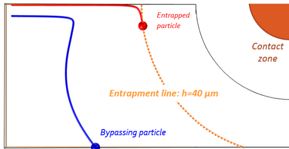
Figure 1: Numerical model
