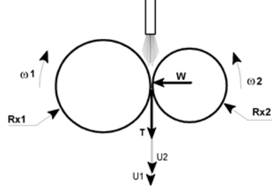
Figure 1: Twin-disc machine
