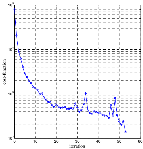
Figure 3. Cost-function evolution without measurement noises
