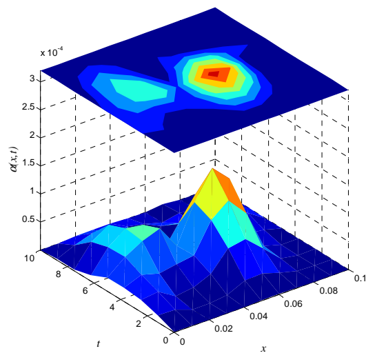
Figure 6. Identified thermal diffusivity at iteration 7.
