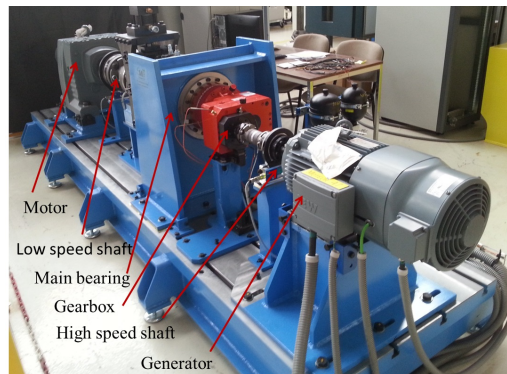
Figure 1: Experimental test bench
