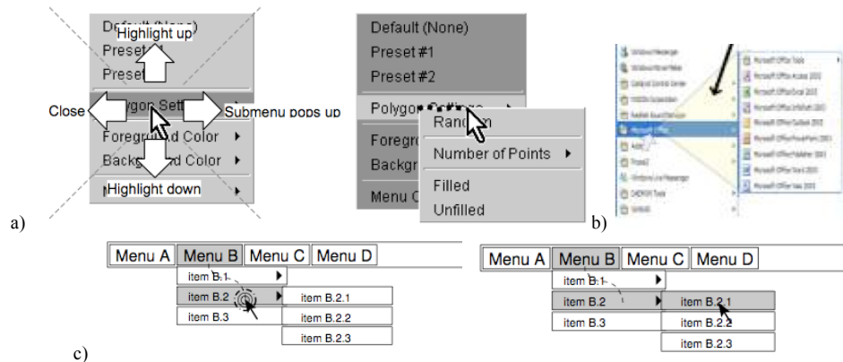
Figure 14: a) Motion menu [Kobayashi et Igarashi 2003], © ACM, an horizontal cursor movement opens/closes submenus at the position where the horizontal movement occurs. Vertical movements are only used to highlight the item under the cursor. b) AAMUs [Tanvir et al. 2008], © ACM, display submenus at mid-height and provides an enlarged activation area to make it easier to reach submenus. This area, which is triangular-shaped, partially overlaps the parent menu. While the cursor is over this area, the submenu remains open. c) Jumping menus [Ahlström et al. 2006], © ACM, warp the cursor to the submenu when the user clicks on its parent item, so that the cursor "jumps" from the item to its submenu.
