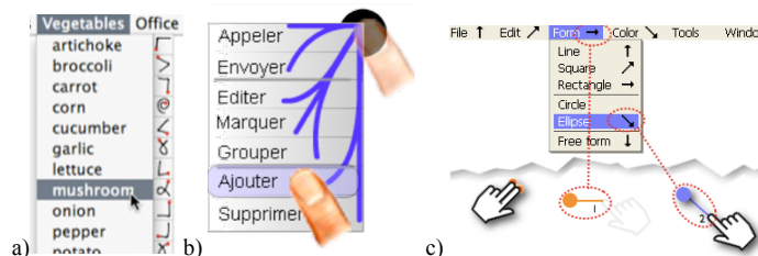
Figure 21: Command-gesture mapping displayed a) [Appert et al. 2009], b) Leaf menus [Roudaut et al. 2009], c) Radial-Stroke shortcuts [Bailly et al 2010], @ACM.
