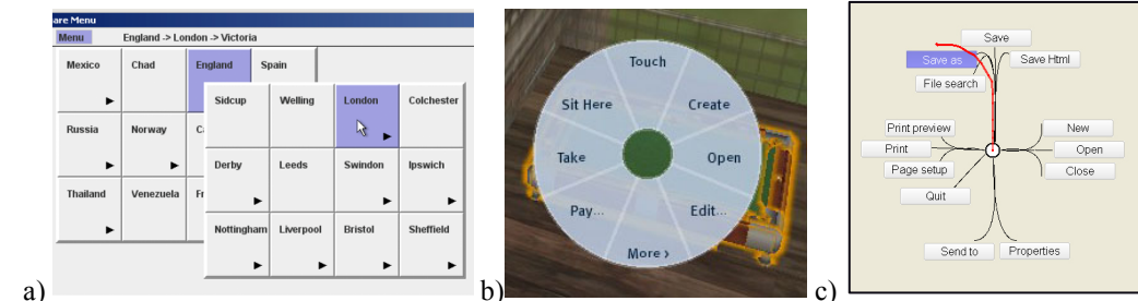
Figure 13: a) Square menus [Ahlstrom et al. 2010], © ACM, organize items in a matrix. b) Pie menus [Callahan et al. 1988], © ACM, place items in a circular design at an equal radial distance from the center (radial layout). c) Flower menus [Bailly et al. 2008] are a variant of Marking menus which rely on curved gestures to increase the number of commands.
