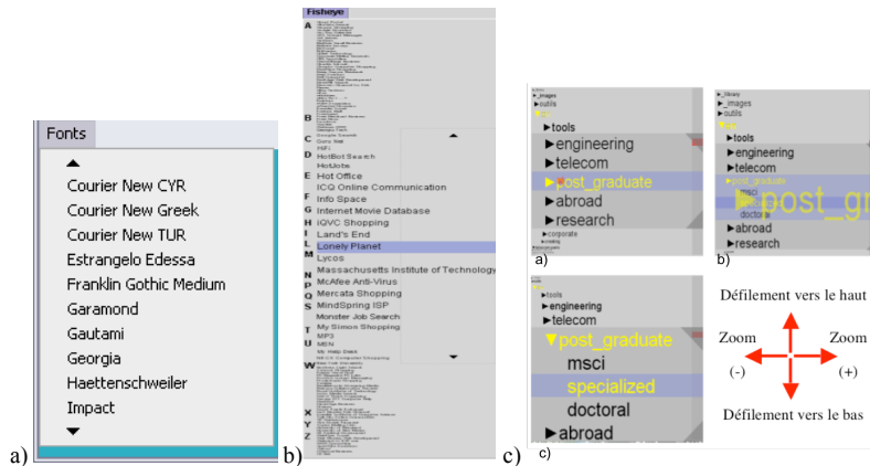
Figure 18: a) Scrollable menu . 2 scroll buttons enable the access to previous or next items. b) Fisheye menu [Bederson 2000], © ACM. The size of items dynamically changes relatively to their degree of interest (DOI): items located in the focus area (with a high DOI) are displayed at a readable size while the size of the items lying in the context area is inversely proportional to their distance from the focus zone. c) FishTree [Lecolinet and Nguyen. 2006] extends the Fisheye menu for hierarchical menus.
