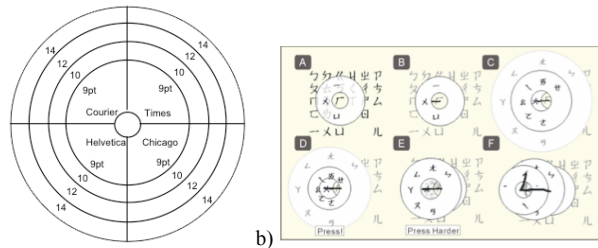
Figure 17: a) DartBoard menus in a) [Kurtenbach 1993], increase menu breadth by combining orientation and distance. b) Donut menu [Lai et al. 05, Ren et al. 08] combine orientation and 2 or 3 levels of pressure.
