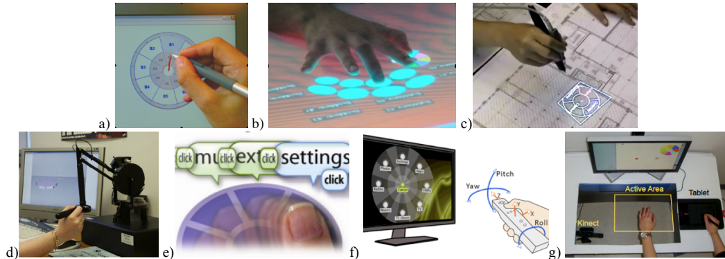
Figure 8: Menu using non-traditional input/output capabilities. a) Push menus use pressure input [Huot et al. 2008]. b) MTM uses multi-finger inputs [Bailly et al. 08], © ACM. c) Marking menu using a pen with a pico-projector [Song et al. 2009], © ACM. d) HardBorder uses haptic feedback [Essert-Villard and Capobianco 2009], © ACM. e) EarPod uses audio feedback [zhao et al. 2007], © ACM. f) TV Menus using a gesture-aware remote control [Bailly et al. 2011]. g) Two-handed Marking menus are a near-surface menu [Guimbretière and Nguyen 2012], © ACM.
