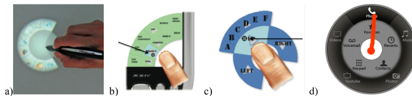
Figure 7: a) Occlusion aware menus [Brandl al. 2009], © ACM; some items are left empty to avoid occlusion. b) Arch Menu and c) ThumbMenu [Huot et al. 2007] use an offset cursor to improve finger selection accuracy with small items. d) Wavelet menus [Francone et al. 2010] place submenus at the center of the menu to fit small screens without degrading navigation, @ACM.
