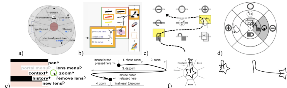
Figure 6: a) Users can make the submenus persistent with the Floating Pie menus [Rubio and Janecek 2002]. b) CrossY [Apitz et al. 2004], c,d) Grid gates and Polar gates [Sulaiman et al. 2008] allow users to compose several commands by performing a single gesture. e) Control menus [Pook et al. 2000] allow users to select a command and control a parameter in the same gesture.
