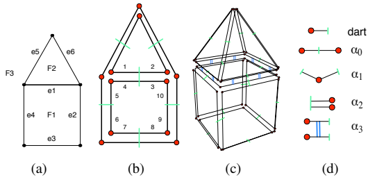
Figure 1: n-Gmap representations. (a) A 2D object containing 3 faces, 6 edges and 5 vertices. (b) Corresponding 2-Gmap: the set of darts {1,2,3,4} represents edge e_1 , the set of darts {3,4,5,6,7,8,9,10} represents face F_1 . (c) 3D object composed of 2 volumes represented with 3-Gmap. (d) Symbolic representation of involutions.
