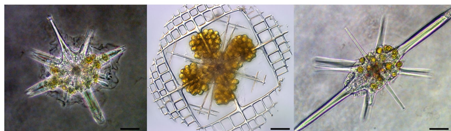
Figure 1. Microscopic pictures of symbiotic Acantharia that harbor 10 to 100 symbiotic microalgae (yellow cells) in their cytoplasm. Scale bars = 20 \mu\text{m} .
