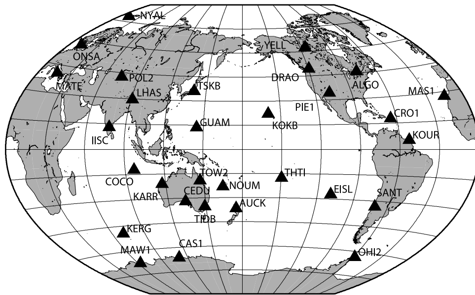
Figure 4. International GNSS Service (IGS) GPS station network used for defining our reference system (30 stations in addition to the local network).
