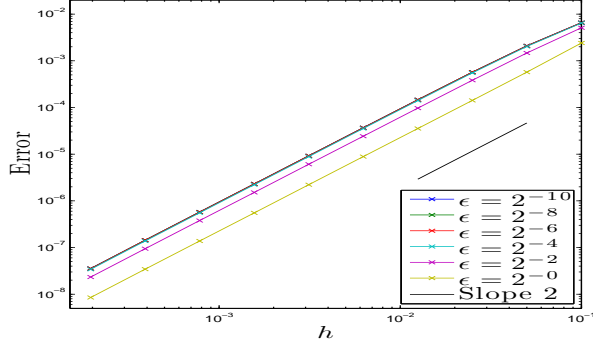
(a) err_{(S^\epsilon, A^\epsilon)}(T_f = 0.2) w.r.t h , N_x = 2^8
