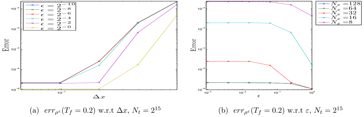
FIGURE 4. Error on the density \rho^\epsilon for the splitting scheme (1.17) of order 1 before the caustics: dependence on \epsilon and on \Delta x .
