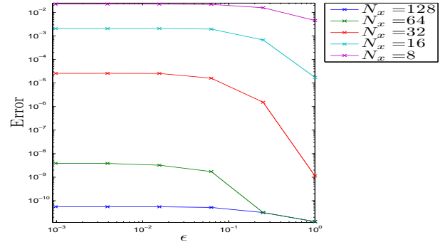
(b) err_{\rho^\varepsilon}(T_f = 0.2) w.r.t \varepsilon , N_t = 2^{15}
