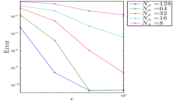
(b) err_{\rho^\varepsilon}(T_f = 1) w.r.t \varepsilon , N_t = 2^{17}
