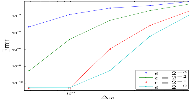
(a) err_{\rho^\varepsilon}(T_f = 1) w.r.t \Delta x , N_t = 2^{17}
