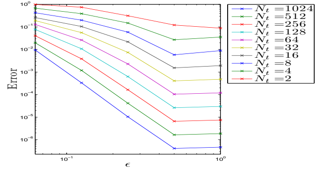
(b) err_{\rho^\varepsilon}(T_f = 1) w.r.t \varepsilon , N_x = 2^8
