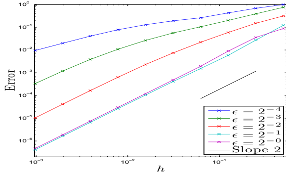
(a) err_{\rho^\varepsilon}(T_f = 1) w.r.t h , N_x = 2^8
