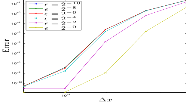
(a) err_{\rho^\epsilon}(T_f = 0.2) w.r.t \Delta x , N_t = 2^{15}
