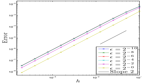
(a) err_{(S^\varepsilon, A^\varepsilon)}(T_f = 0.2) w.r.t h , N_x = 2^8
