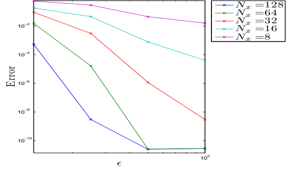
(b) err_{\rho^\epsilon}(T_f = 1) w.r.t \epsilon , N_t = 2^{17}
