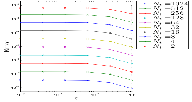
(b) err_{(S^\varepsilon, A^\varepsilon)}(T_f = 0.2) w.r.t \varepsilon , N_x = 2^8
