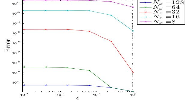
(b) err_{\rho^\epsilon}(T_f = 0.2) w.r.t \epsilon , N_t = 2^{15}
