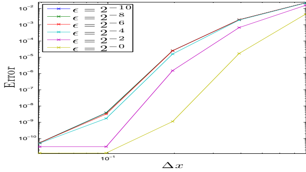
(a) err_{\rho^\varepsilon}(T_f = 0.2) w.r.t \Delta x , N_t = 2^{15}
