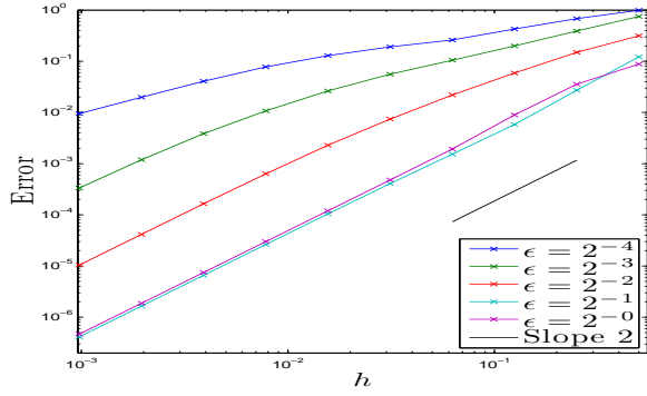
(a) err_{\rho^\epsilon}(T_f = 1) w.r.t h , N_x = 2^8
