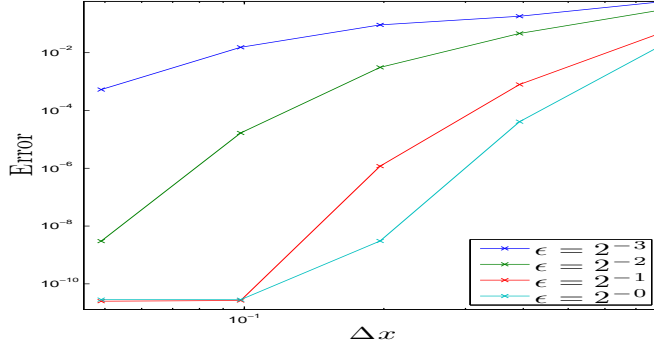
(a) err_{\rho^\epsilon}(T_f = 1) w.r.t \Delta x , N_t = 2^{17}
