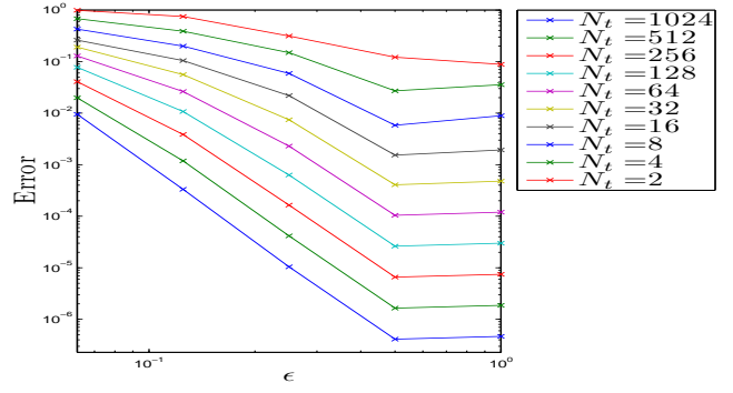
(b) err_{\rho^\epsilon}(T_f = 1) w.r.t \epsilon , N_x = 2^8
