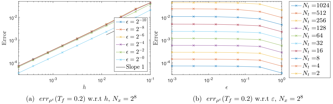
FIGURE 2. Error on the density \rho^\epsilon for the splitting scheme (1.17) of order 1 before the caustics: dependence on \epsilon and on h .
