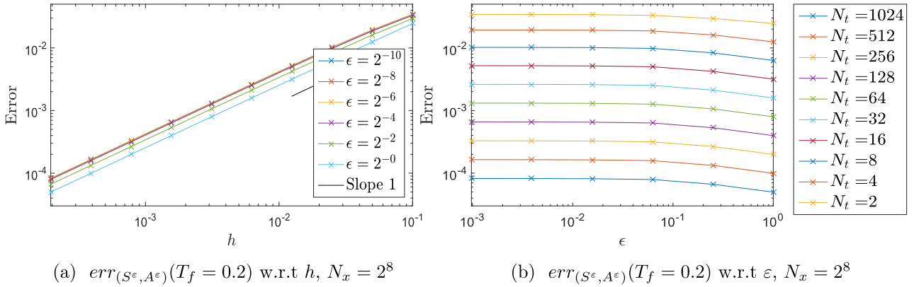
FIGURE 3. Error on (S^\epsilon, A^\epsilon) for the splitting scheme (1.17) of order 1 before the caustics: dependence on \epsilon and on h .
