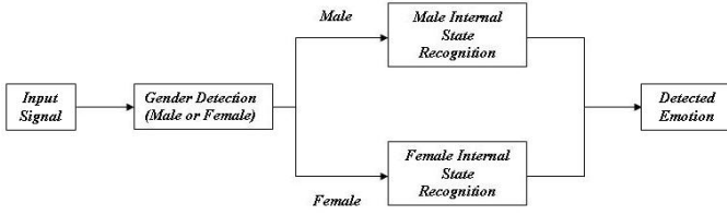
Fig. 3: Combined Gender and Internal States Recognition Architecture
