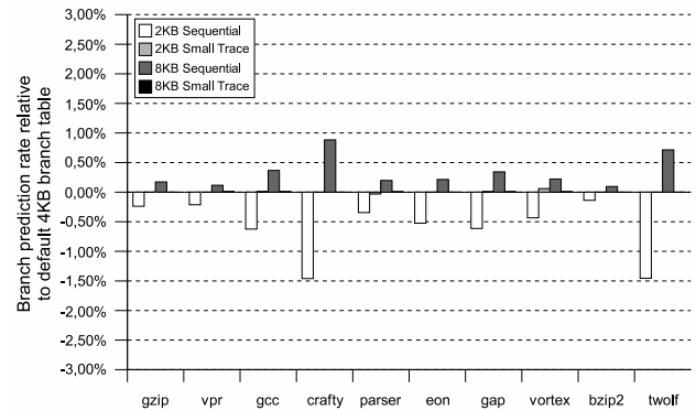
Figure 26: Trace Size Reduction: Varying branch prediction tables size (branch prediction rate); 1 PIII 500.
