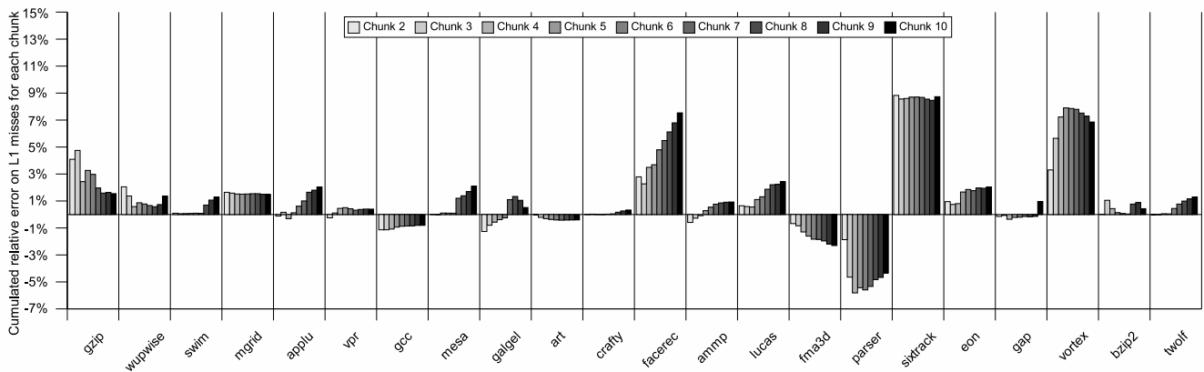
Figure 28: Evolution of global versus local error (L1 miss rate); full set, 10 PIII 500.
