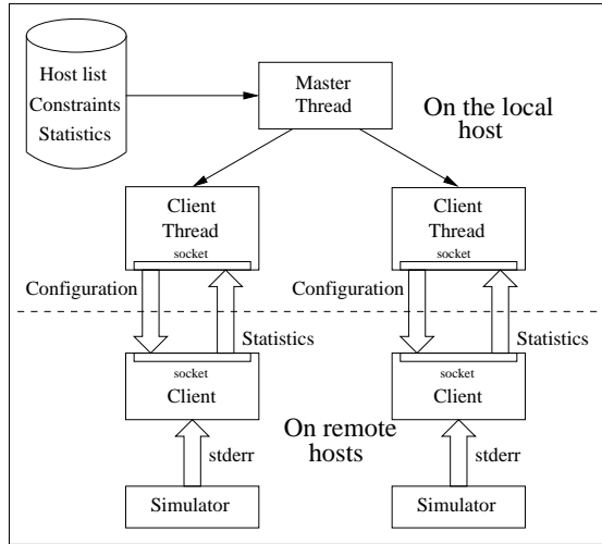
Figure 5: The DiST architecture.
