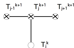
Figure 4.5: The difference stencil of the Euler backward method for the heat equation
