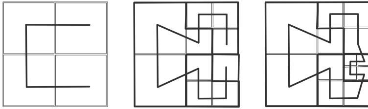
Figure 2.35: Space filling curves, regularly and irregularly refined
