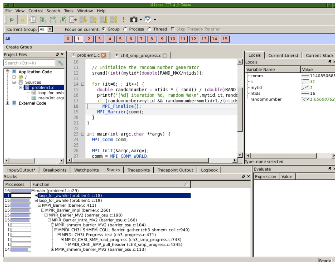
Figure 27.1: Display of 16 processes in the DDT debugger
