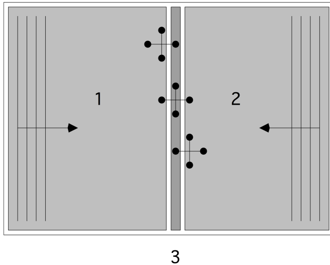
Figure 6.14: Domain dissection into two unconnected subdomains and a separator
