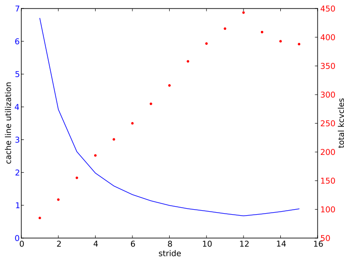
Figure 31.1: Run time in cycles and L1 reuse as a function of stride
