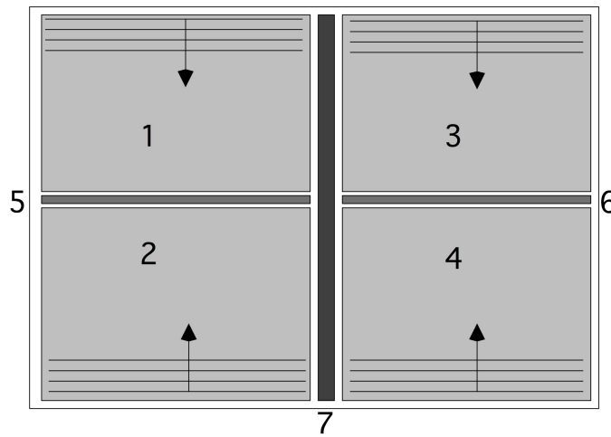
Figure 6.15: A four-way domain decomposition
