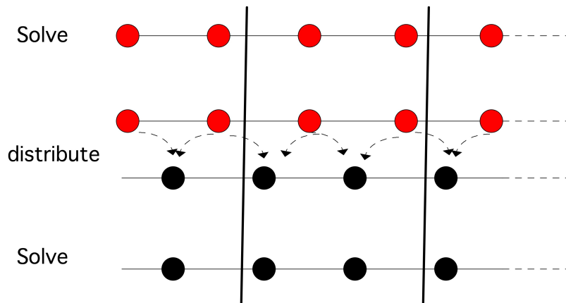
Figure 6.19: Parallel red-black solution on a 1d domain
