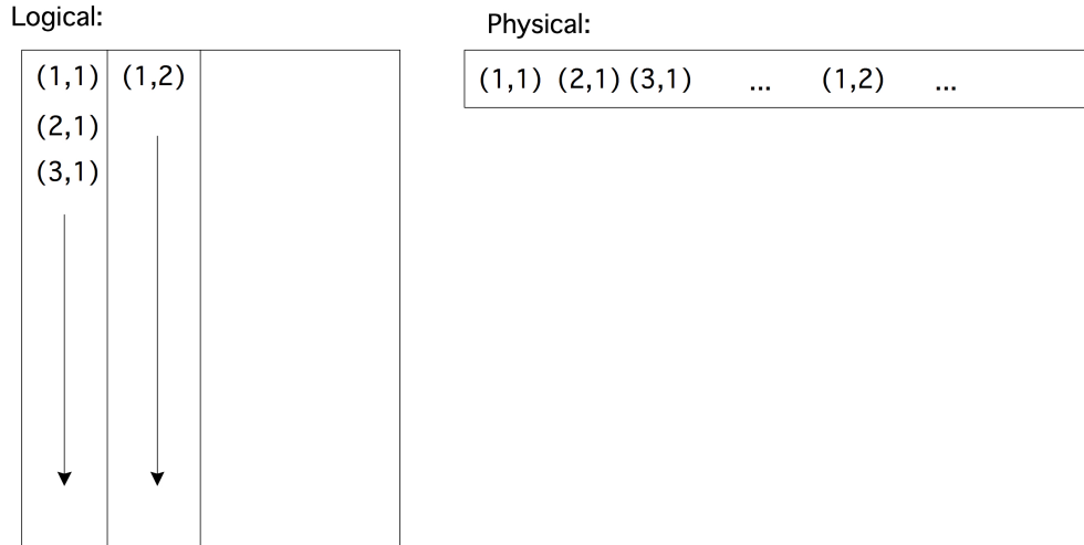
Figure 24.1: Column-major storage of an array in Fortran
