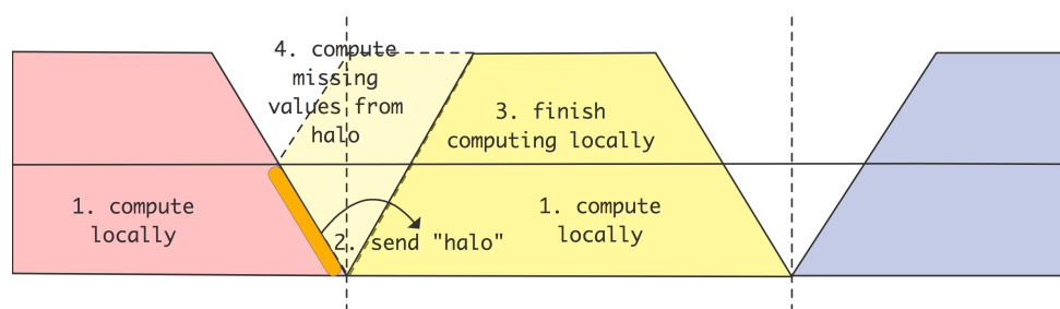
Figure 6.24: Computation of blocks of grid points over multiple iterations
