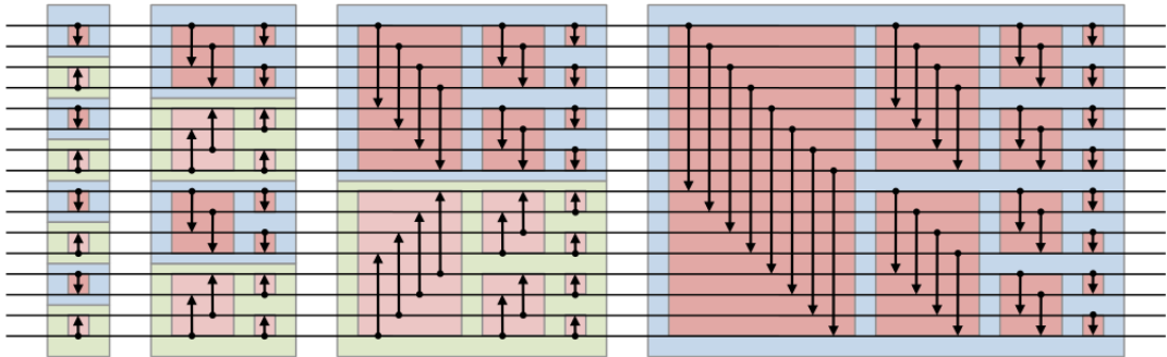
Figure 8.3: Full bitonic sort for 16 elements
