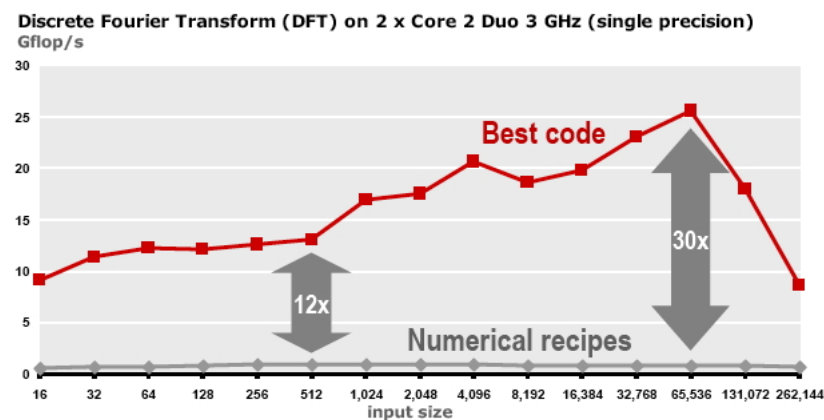
Figure 1.22: Performance of naive and optimized implementations of the Discrete Fourier Transform
