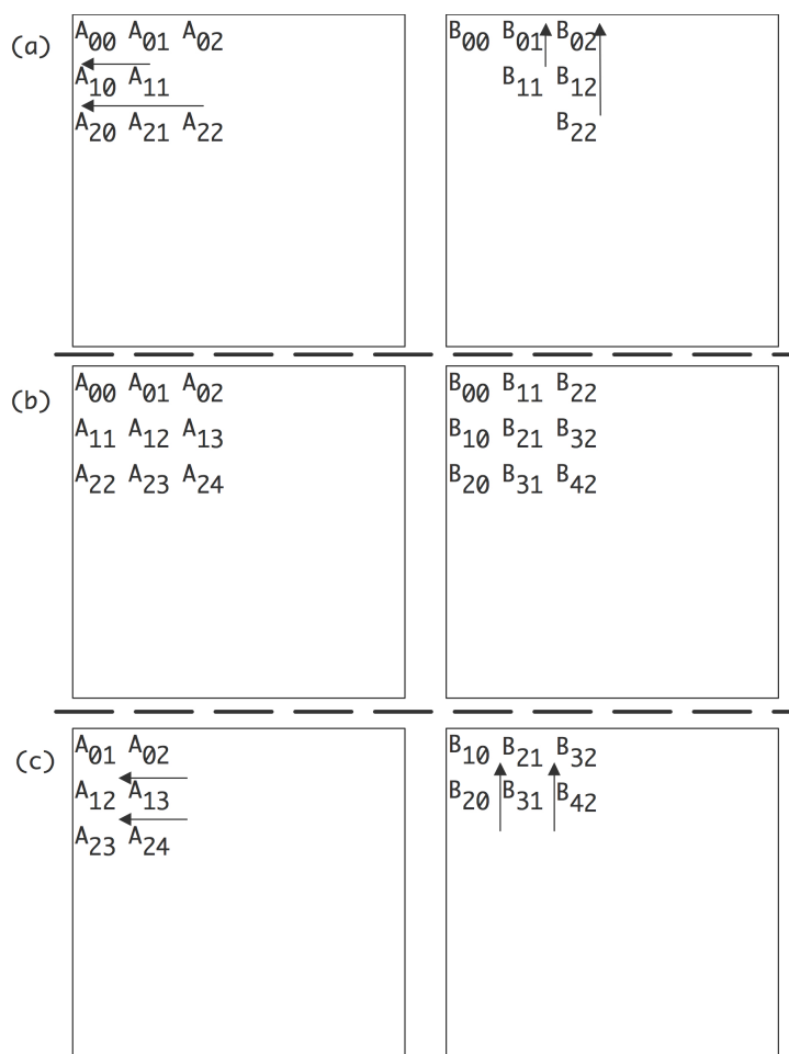
Figure 6.7: Cannon's algorithm for matrix-matrix multiplication: (a) initial rotation of matrix rows and columns, (b) resulting position in which processor (i, j) can start accumulating \sum_k A_{ik} B_{kj} , (c) subsequent rotation of A, B for the next term.
