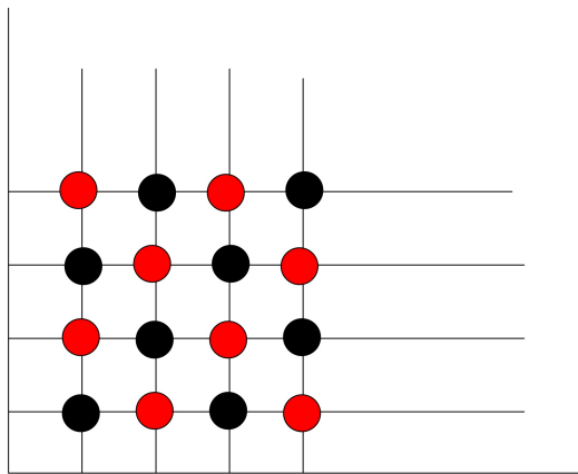
Figure 6.20: Red-black ordering of the variables of a two-dimensional domain
