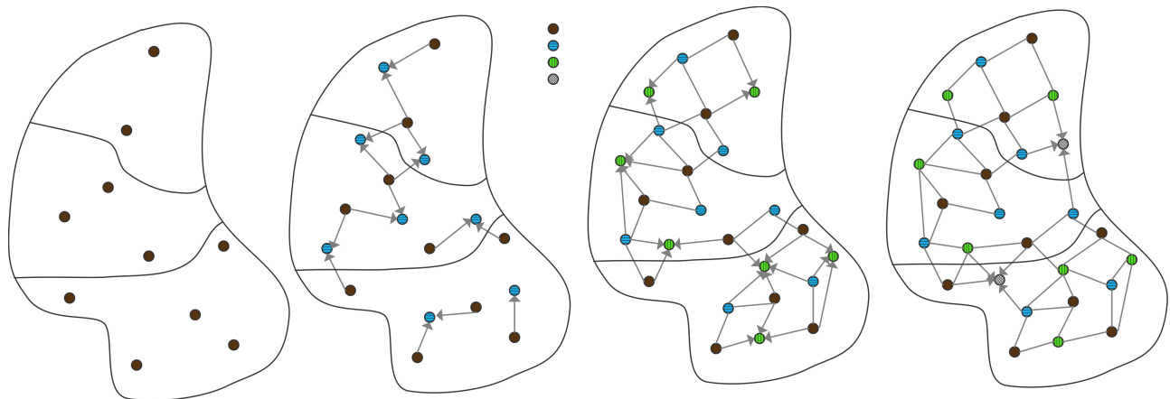
Figure 6.13: Solving a parallel multicolour ILU in four steps
