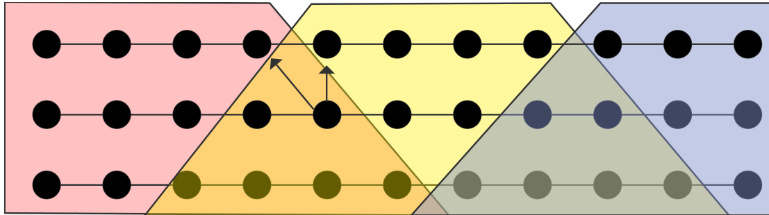
Figure 6.22: Computation of blocks of grid points over multiple iterations
