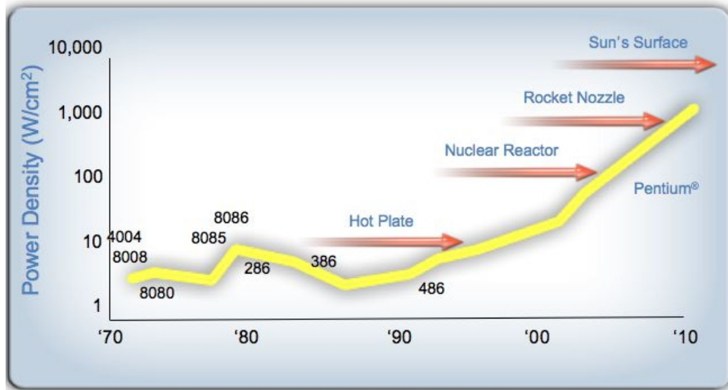
Figure 1.28: Projected heat dissipation of a CPU if trends had continued – this graph courtesy Pat Helsing illustrates the heat that a chip would give off, if single-processor trends had continued.
