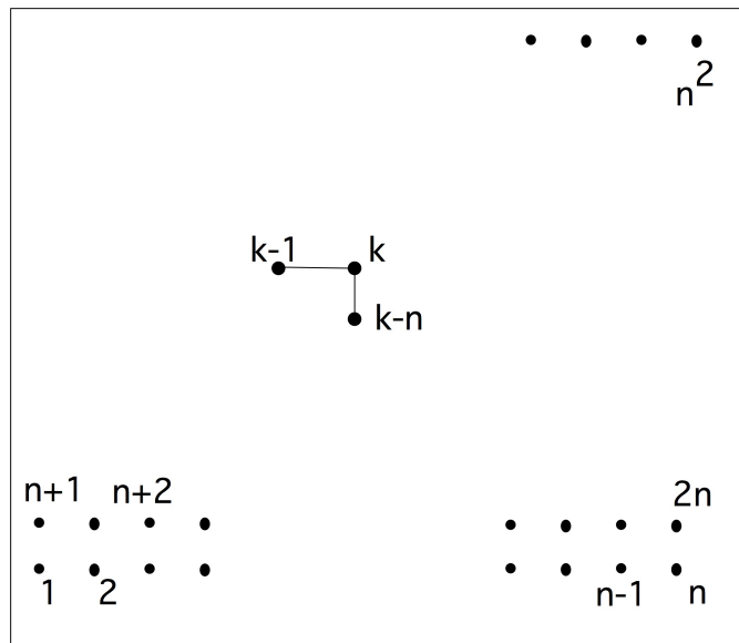
Figure 6.21: The difference stencil of the L factor of the matrix of a two-dimensional BVP
