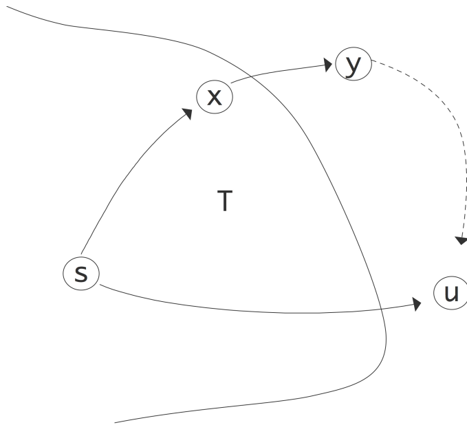
Figure 9.1: Illustration of the correctness of Dijkstra's algorithm
