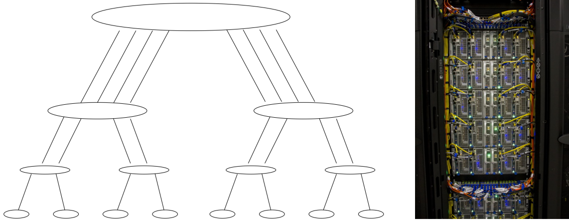
Figure 2.27: A fat tree with a three-level interconnect (left); the leaf switches in a cabinet of the Stampede cluster (right)
