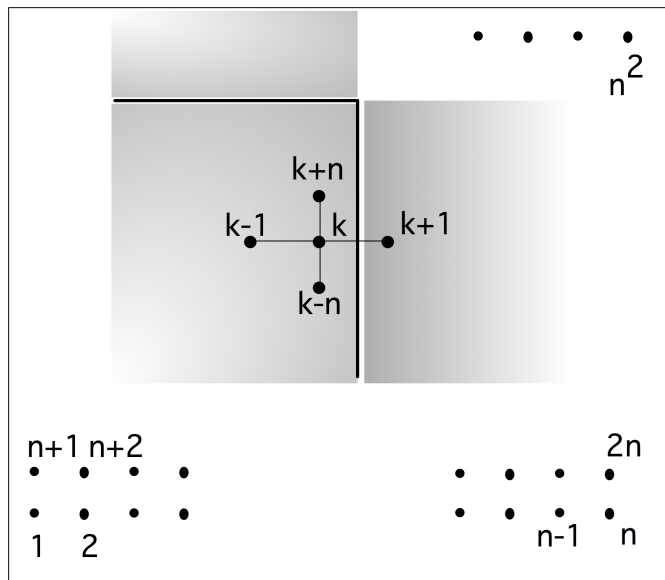
Figure 6.8: A difference stencil applied to a two-dimensional square domain, distributed over processors. A cross-processor connection is indicated.
