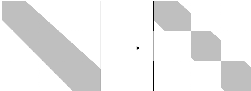
Figure 6.11: Sparsity pattern corresponding to a block Jacobi preconditioner
