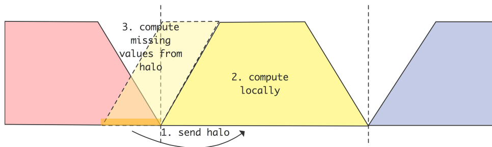
Figure 6.23: Computation of blocks of grid points over multiple iterations
