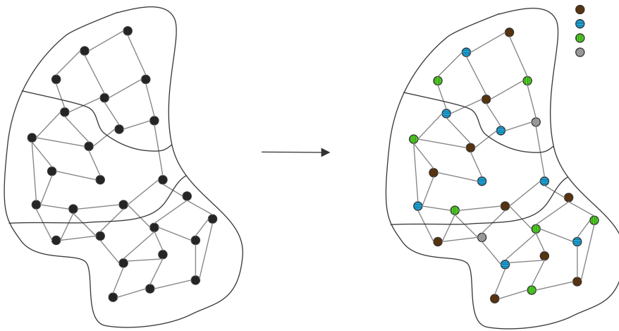
Figure 6.12: A partitioned domain with coloured nodes
