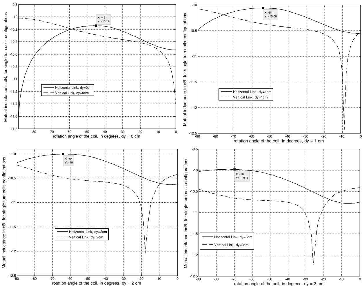
Fig. 6. Mutual inductance in HL (solid line) and VL (dotted line) configuration (7 cm x 7 cm square loop).
