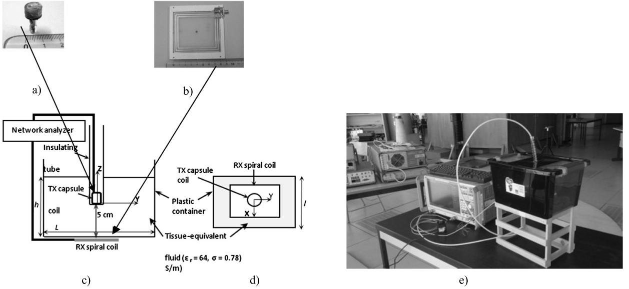
Fig. 12. (a) Fabricated TX multilayer capsule coil; (b) fabricated RX 3-turn receiver spiral coil; measurement set-up: (c) side view; (d) top view; (e) pictures of the measurement set-up.
