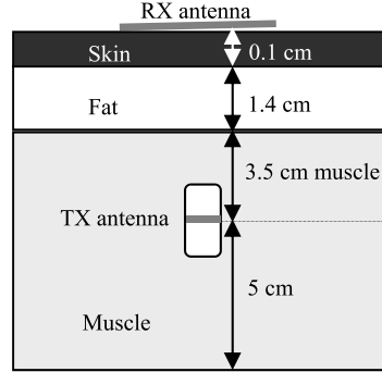
Fig. 9. MI link through a three-layer human body (muscle/fat/skin).
