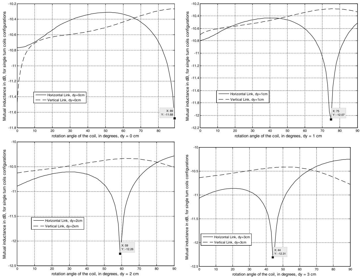
Fig. 5. Mutual inductance in HL (solid line) and VL (dotted line) configuration (4 cm \times 4 cm square loop).
