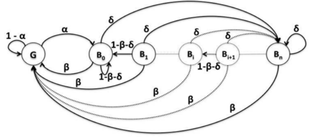
Fig. 15. Discrete Markov chain representation of the RFR service.
