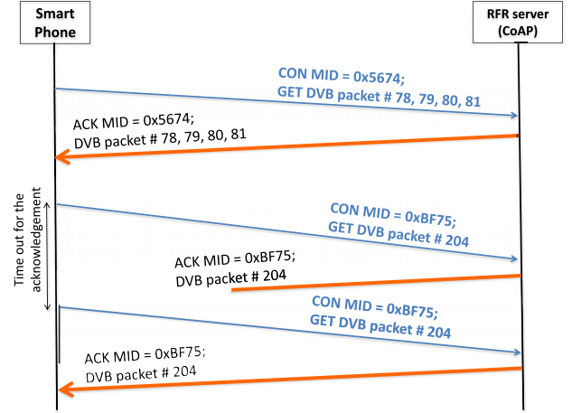
Fig. 3. RFR service via LTE network for a simple implementation of CoAP.
