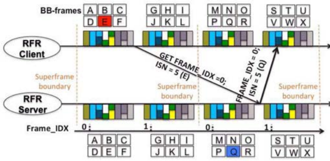
Fig. 6. Ambiguous identification of BB-frame due to large cellular transmission delay.
