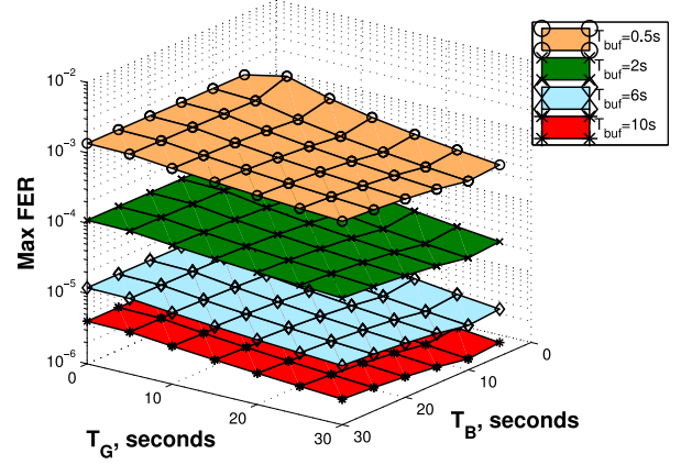
Fig. 18. Maximum FER surfaces for different values of T_G & T_B and T_{buf} .
