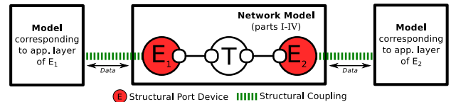
Figure 5. Structural Coupling.
