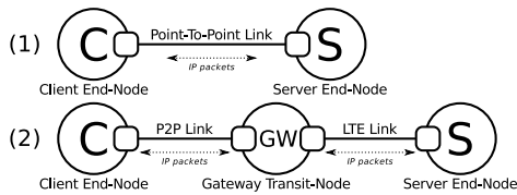
Figure 7. Network topologies corresponding to our PoC, modeling a ping between two nodes, via a P2P link and a LTE infrastructure.
