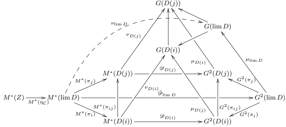
Fig. 2. Commutation of normalisation and Dirichlet averaging
