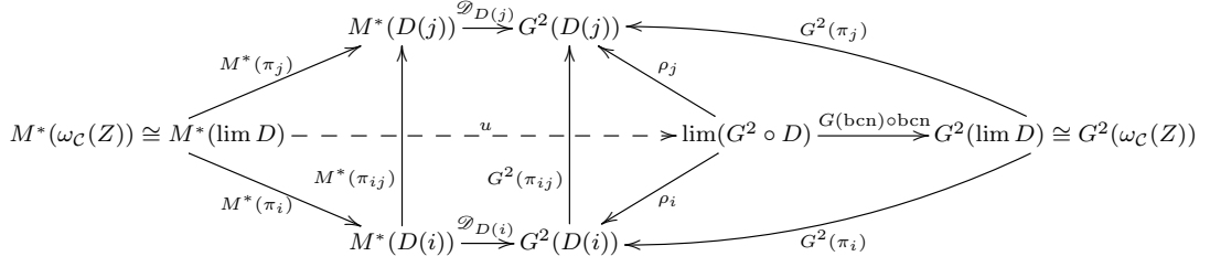
Fig. 1. Construction of \hat{\mathcal{D}} on \omega_{\mathcal{C}}(Z)
