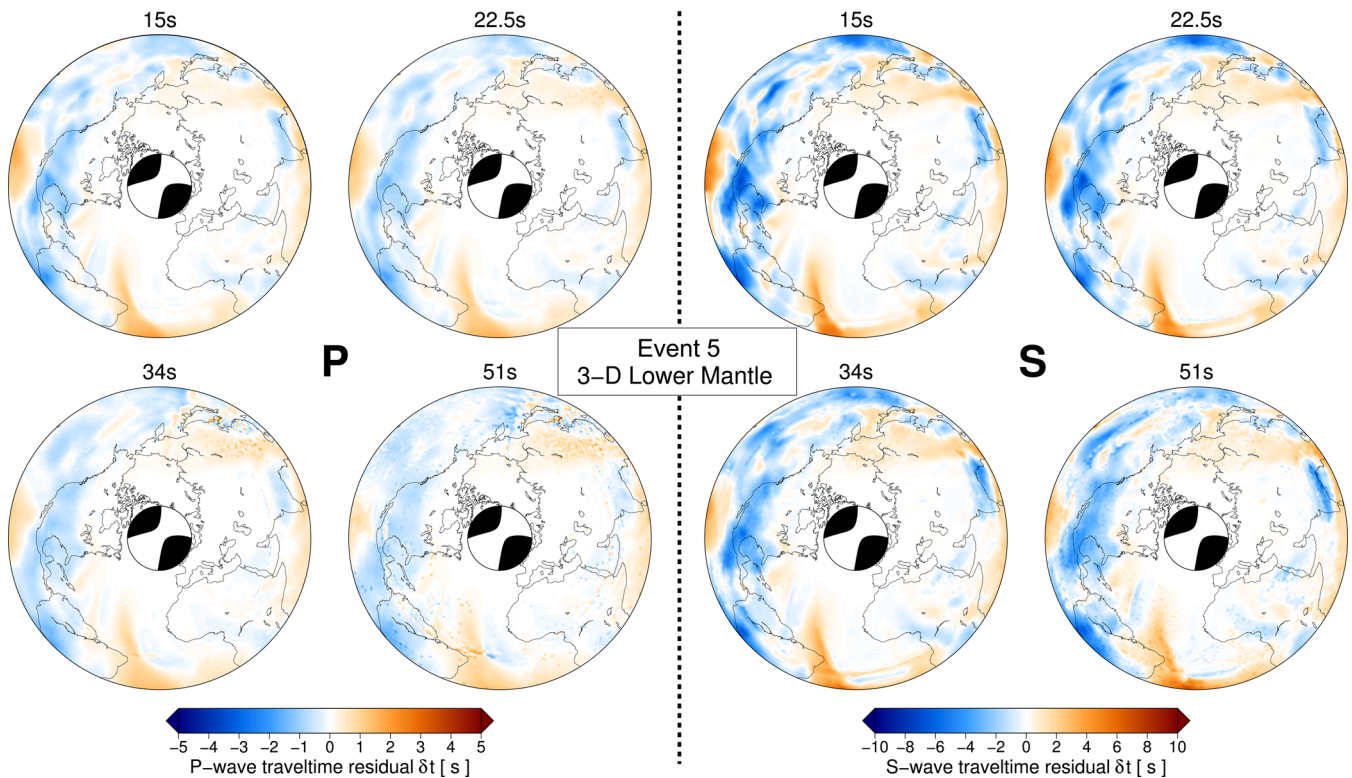
Figure 4. Same as Fig. 2 for the lower-mantle model S09-M2-Q-LM (3-D heterogeneity below 800 km depth only). Note the generally smaller magnitudes of traveltime residuals and the reduced dominance of positive delays compared to the whole-mantle model.
