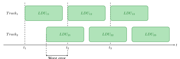
Fig. 3. Example of a constant sampling rate model. First track contains perfectly synced LDUs with the expected timings. The second track exhibits the worst precision, LDUs are exactly in between two expected timings.
