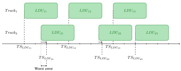
Fig. 4. Example of a timestamp model. First track contains perfectly synced LDUs with the reference clock. Second track exhibits the worst precision when LDU_{21} is exactly in between two reference clock ticks. Arrows show the rounded timestamp.
