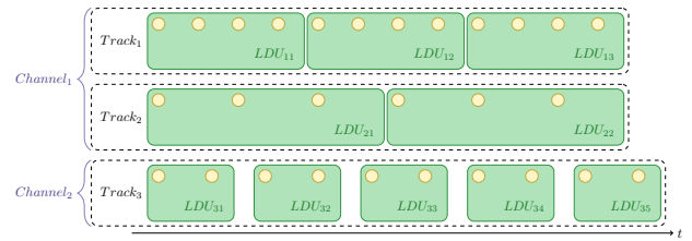
Fig. 2. Multimedia encapsulation, this example showcases two channels containing 2 tracks and 1 track respectively. In track one, each LDUs contain 4 samples, in track two each contains 3 samples each and in track three each contain 2.
