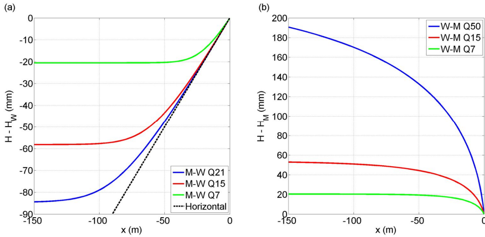
Figure 10: Water depth (modelled) upstream from a roughness transition meadow-to-wood (a) and wood-to-meadow (b).
