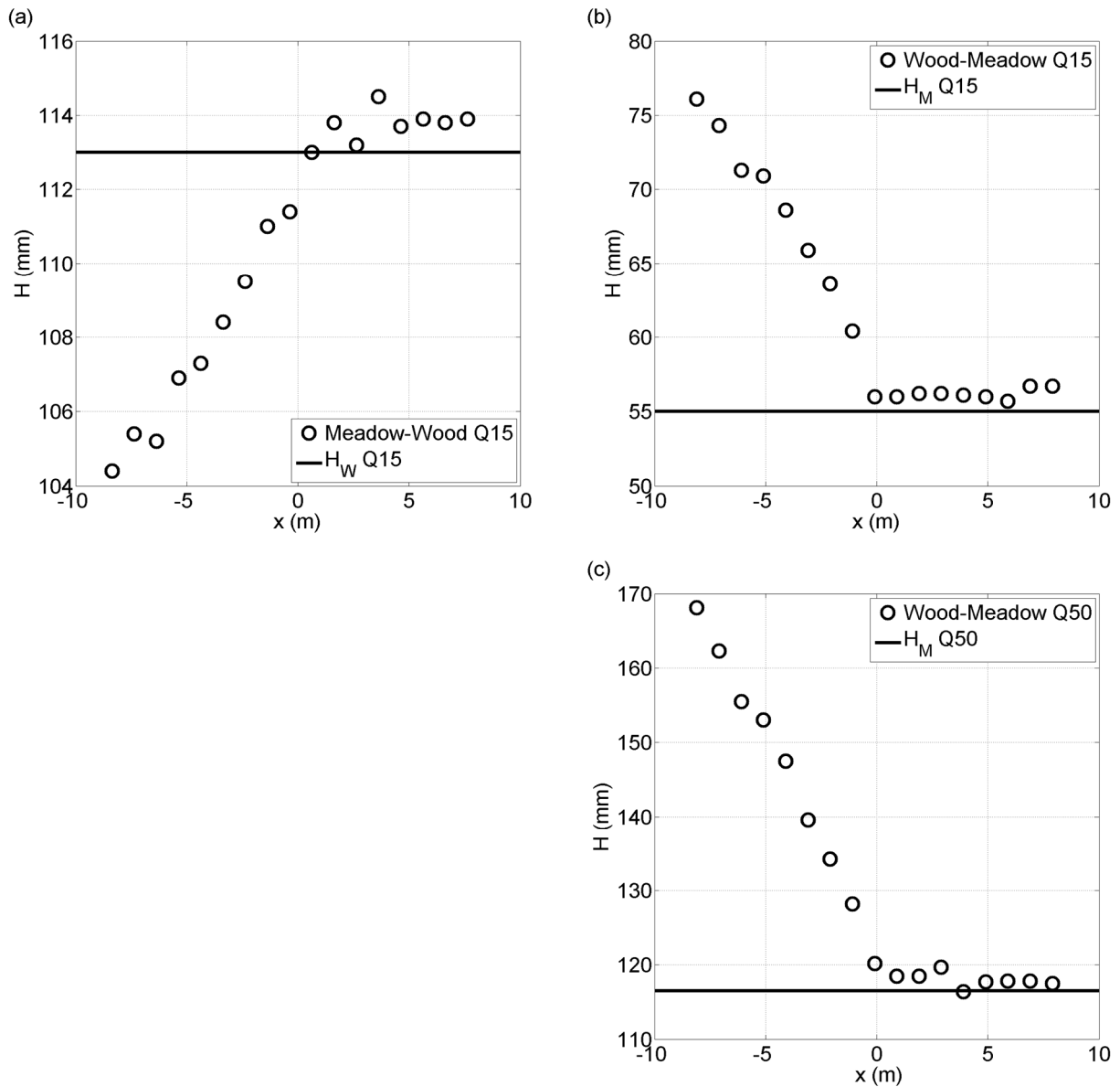
Figure 2: Water depth throughout the meadow-to-wood transition Q = 15 L \cdot s^{-1} (a) and throughout the wood-to-meadow transition Q = 15 L \cdot s^{-1} (b) and Q = 50 L \cdot s^{-1} (c). The solid line is the uniform flow depth of the downstream roughness.
