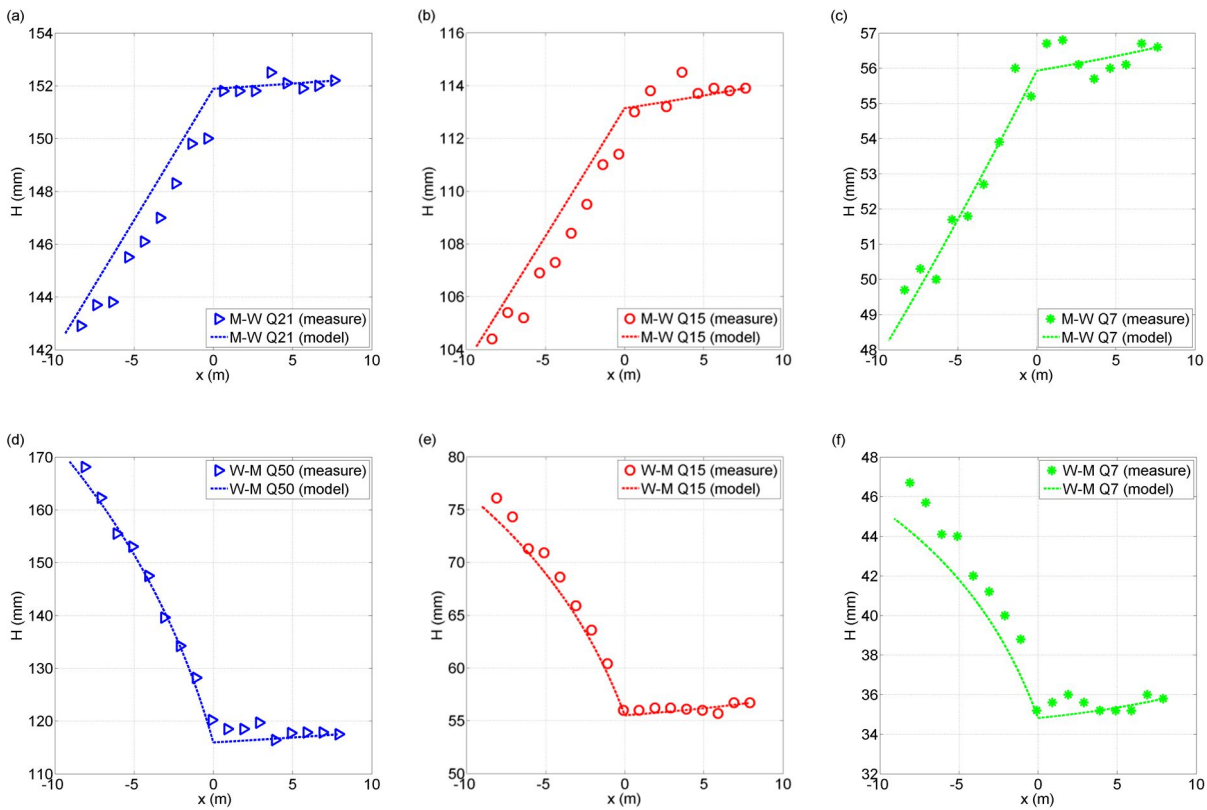
Figure 9: Water depth for transition meadow-to-wood (M-W) [(a): Q = 21 \text{ L}\cdot\text{s}^{-1} ; (b): Q = 15 \text{ L}\cdot\text{s}^{-1} ; (c): Q = 7 \text{ L}\cdot\text{s}^{-1} ] and wood-to-meadow (W-M) [(d): Q = 50 \text{ L}\cdot\text{s}^{-1} ; (e): Q = 15 \text{ L}\cdot\text{s}^{-1} ; (f): Q = 7 \text{ L}\cdot\text{s}^{-1} ].
