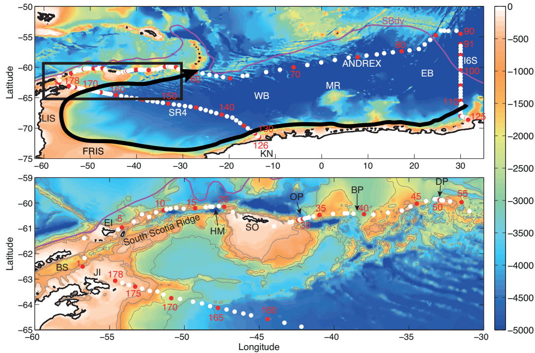
Figure 1. Top panel: Map and bathymetry (from GEBCO) of the Weddell Gyre region showing the 3 sections used in this study (ANDREX, I6S, SR4). For each section, the first and last stations as well as every fifth stations are shown in red. The Southern Boundary of the ACC in magenta; the Weddell Gyre is indicated schematically by the black arrow. From left to right, LIS: Larsen Ice Shelves; FRIS: Filchner-Ronne Ice Shelves; KN: Kapp Norvegia; WB: Weddell Basin, MR: Maud Rise, EB: Enderby Basin. Bottom panel: detailed map of the South Scotia Ridge (black rectangle in top panel). From left to right, BS: Bransfield Strait; JI: Joinville Island; EI: Elephant Island; HM: Hesperides Mouth; SO: South Orkney Islands; OP: Orkney Passage; BP: Bruce Passage; DP: Discovery Passage.
