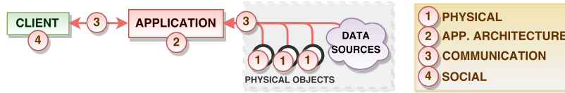
Figure 1: A typical WoT app architecture and its context dimensions
