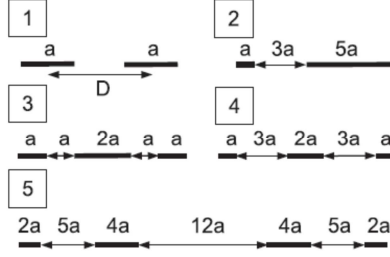
Fig. 7. Some cases of unions of segments.
