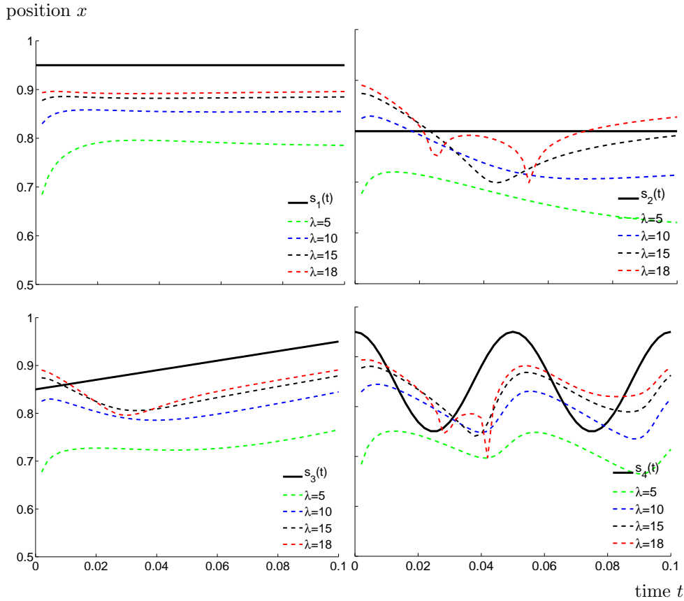
FIG. 7.1. Test conductivities and their reconstructions; the vertical axis is the variable x , the horizontal axis is the time t . Solid black line is the boundary s_i(t) , dashed lines are the reconstructions with \lambda = 5, 10, 15, 18 . On top left: s_1(t) = 0.95 . On top right: s_2(t) = 0.8 . On bottom left: s_3(t) = 0.85 + t . On bottom right: s_4(t) = 0.85 + 0.1 \cos(t/0.1 \cdot 4\pi) .
