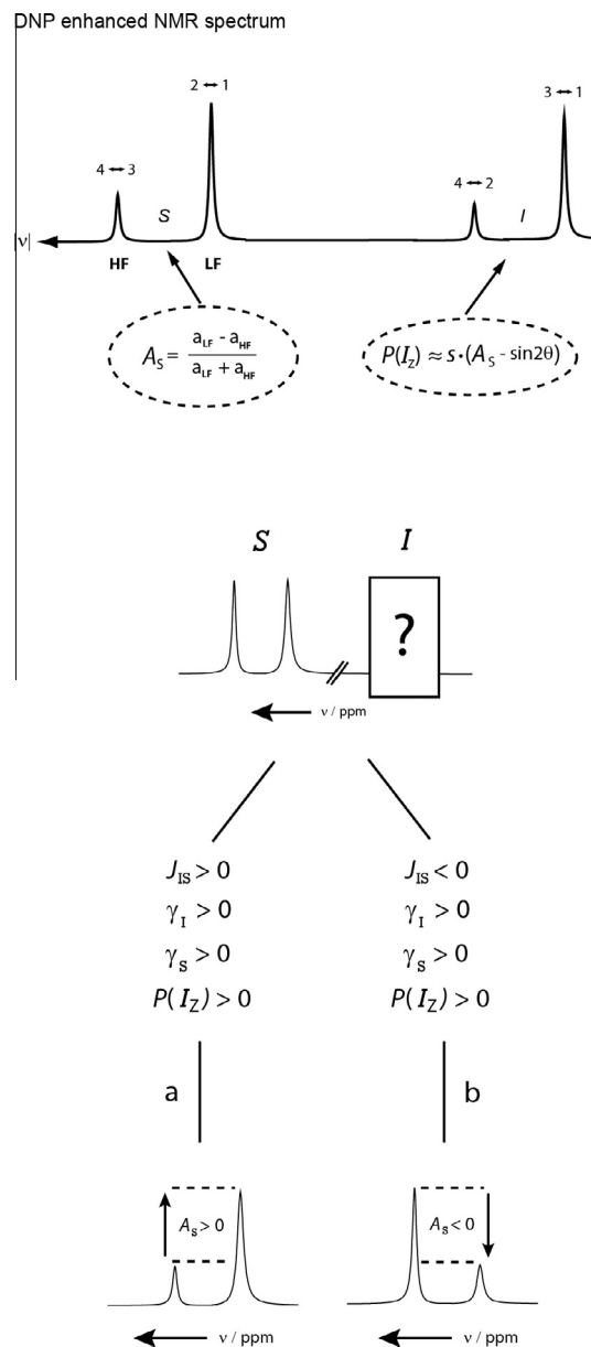
Fig. 2. Illustration of an NMR spectrum of an arbitrary pair of coupled spins I and S enhanced by dissolution DNP. Two examples of the 2^4 possibilities for a coupled two-spin system are shown with their respective asymmetries. The same pattern as b is obtained if an odd number of the parameters \{\gamma_I, \gamma_S, J_{IS}, P(I_z)\} has a negative value. Thus the absolute sign of J_{IS} can readily be determined.
