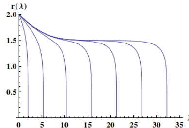
FIG. 2. The area coordinate r , in m = 1 units, as a function of the volume parameter \lambda , obtained integrating the equation (17). As A \rightarrow A_c , \lambda_f = V/4\pi \rightarrow \infty .
