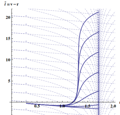
FIG. 6. The family \Sigma_0 in a Reissner-Nordström black hole for M = 1 and Q = 0.7 . The inner (apparent) horizon is at r_- \approx 0.29 and the outer (event) horizon at r_+ \approx 1.71 . We have taken v_f = 0
