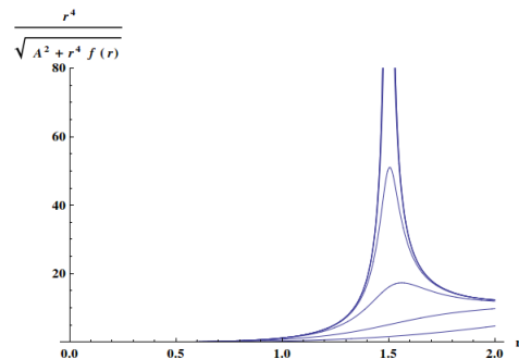
FIG. 3. The integrand in (19) for different values of A gradually approaching A_c . As A \rightarrow A_c the volume contribution comes increasingly from r_V = 3m/2 .
