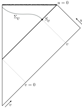
FIG. 1. Conformal diagram of a collapsing object spacetime. The sphere S_v is on the horizon, at time v . The spacelike surface \Sigma_v whose volume we are computing is the one of maximum volume among those bounded by S_v .
