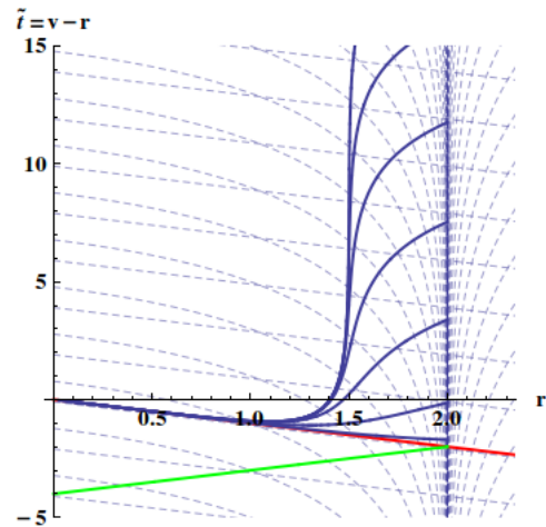
FIG. 5. The maximal volume surfaces inside a black hole formed by a collapsing object. In red is an incoming spherical null shell that collapses and forms a singularity at v = 0 . (The region below the null shell is flat.) As (asymptotic) time passes, the interior grows. In green is the horizon.
