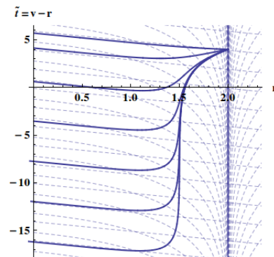
FIG. 4. Black hole spacetime in Eddington-Finkelstein coordinates. The horizon is the vertical line r = 2m . Dashed lines are the null geodesics. Maximum volume surfaces for different values of A , starting from the same sphere on the horizon are depicted.
