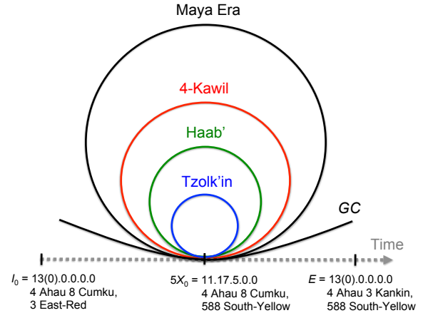
FIG. 1. Mayan/Aztec cyclical vs linear concept of time, with the 260-day Tzolk'in, the 365-day Haab', the 3276-day 4-Kawil, the Maya Era of 13 Baktun (5125 years) and the grand cycle \mathcal{G}\mathcal{C} of 511 Maya Eras. The mythical date of creation \mathcal{I}_0 (11 August 3114 BC), the date corresponding to the Itza prophecy 5\mathcal{X}_0 (3 July 1564 CE) and the end of the previous Maya Era \mathcal{E} (21 December 2012) are also represented.
