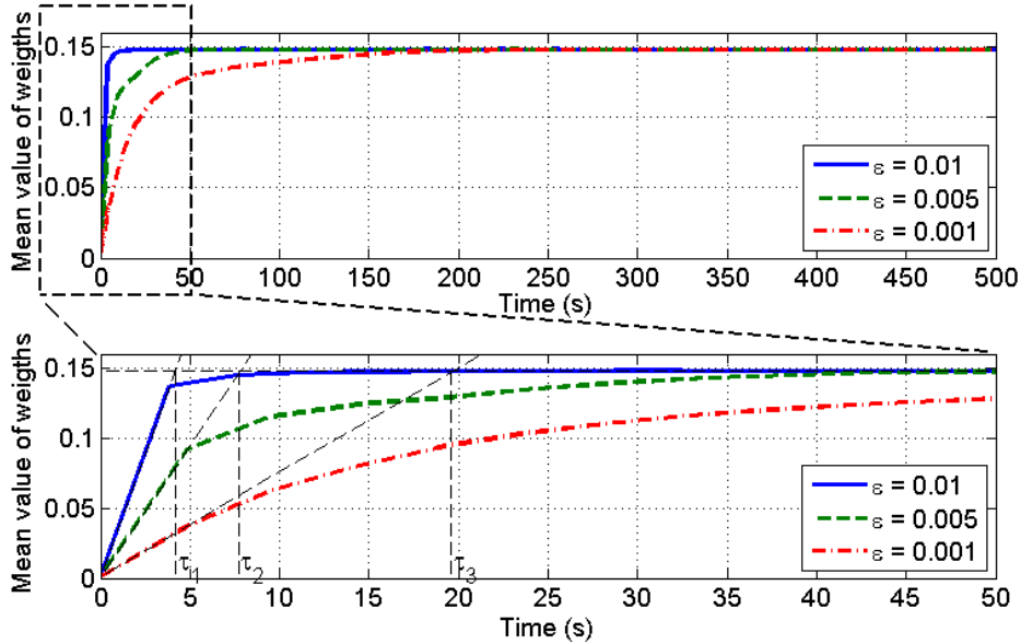
Figure 8. Convergence rate of the Kohonen network during the learning stage based on the mean value of the weights and for different learning steps \epsilon = 0.01, 0.005 and 0.001 . Although the convergence rate is faster for the bigger \epsilon , the networks that slowly adapt to the input matrices are also more finely tuned, as it can be seen in the evolution of the entropy value over the weights, which is also a measure of information or complexity within the network.
