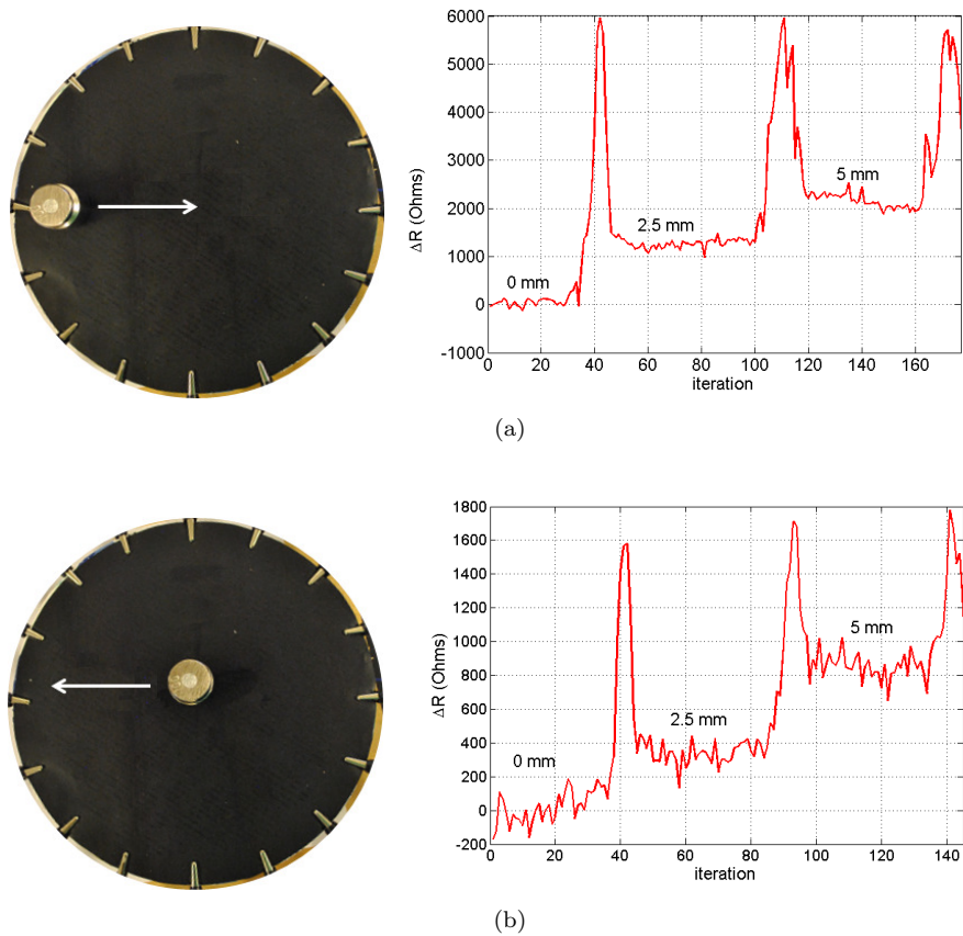
Figure 5. Time series of the ohmic variation \Delta R of the conductive material with respect to spatial displacement (in mm) of a weight of 100g forward and backward; resp. (a) and (b).
