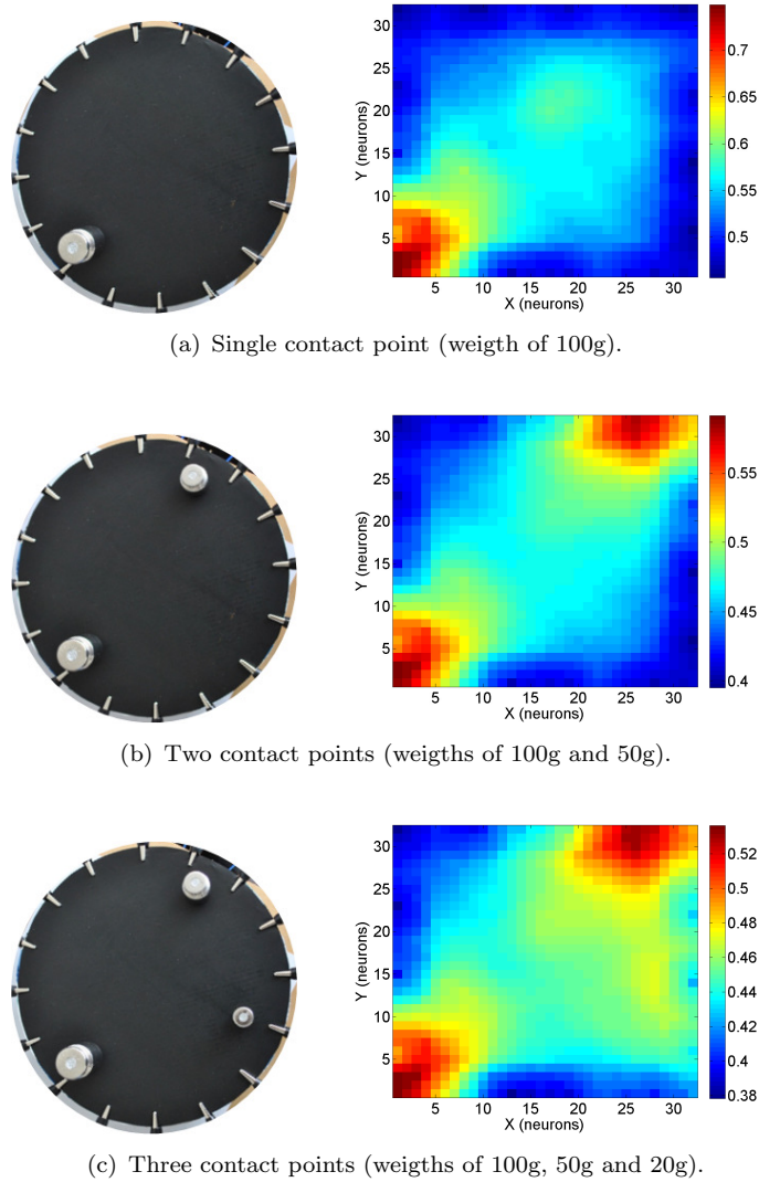
Figure 12. Neural activity of the Kohonen map for multi-touch task for one, two or three weights of 100g, 50g and 20g; resp (a), (b) and (c). The neurons are able to estimate correctly and simultaneously objects of different location and weights.
