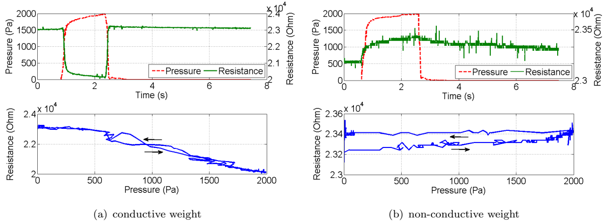
Figure 2. Comparison of the piezo-resistive properties of the conductive material to conductive and non-conductive objects; resp. (a) and (b) for the same weight 100g. On the top chart, the pressure value in Pa at the contact point and the ohmic value of the resistive material. On the bottom chart: Phase plot of the dependence of the material resistance on the pressure. The conductive pressure point shows no hysteresis with respect to the non-conductive pressure point. The ohmic variations also reveal more amplitude for the conductive pressure point (several hundreds of ohms) than the non-conductive one (several dozens of ohms).
