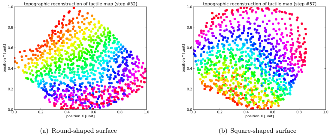
Figure 13. Topological reconstruction from the Kohonen neurons’ synaptic weights using the graphical display based on the Fruchterman-Reingold algorithm for two different type of conductive surface, a round in (a) and a square in (b).
