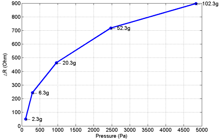
Figure 6. Relation of the variational resistance \Delta R of the conductive material with respect to Pressure ( Pa ) and the weight of objects (same contact point).
