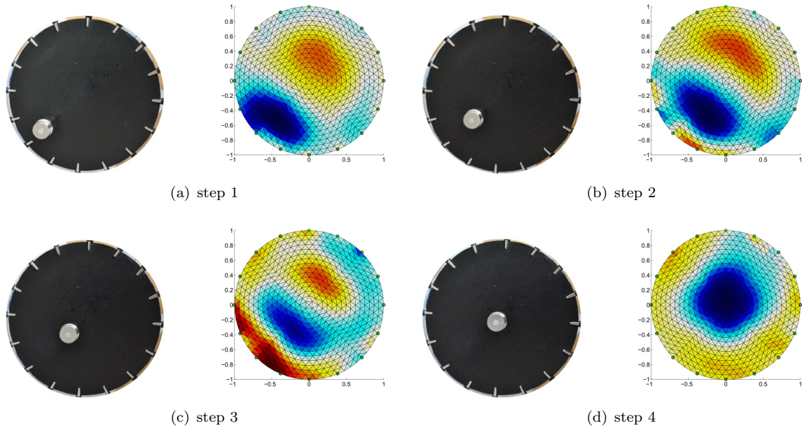
Figure 10. 2 dimensional image reconstruction using EIDORS of a FEM model with 1024 elements. The hyper parameter \alpha (regularization weight) is set to 10^{-3} . Blue and reds areas are the areas with higher and lower resistivity respectively.
