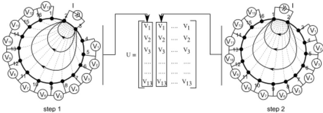
Figure 1. Neighboring method of data collection for EIT showed for a volume conductor and 16 spaced symmetrically electrodes. The voltage is measured 13 times for 16 different injection current, which correspond to the input matrix U of 13 \times 16 = 208 elements.
