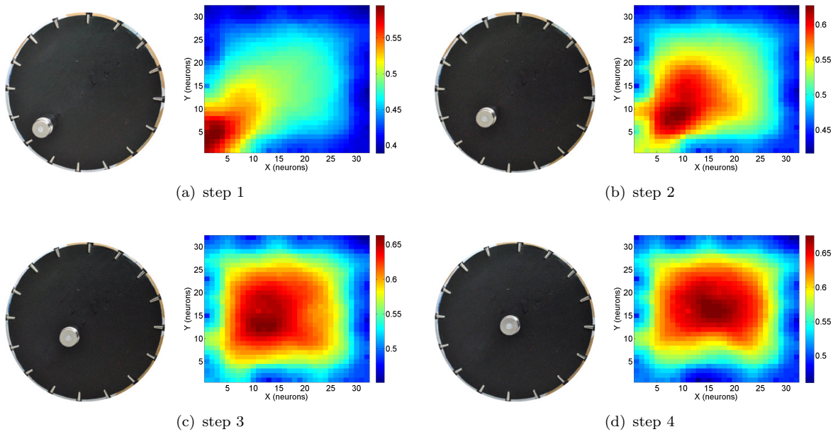
Figure 9. Position of the object (weight = 100g) on the conductive material and the SOM reconstruction (network size 32 \times 32 neurons)
