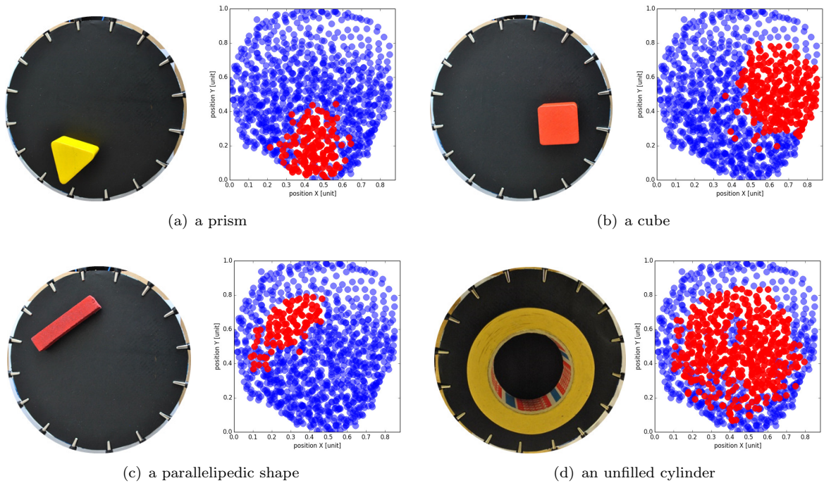
Figure 14. Activity-level of the Kohonen neurons in presence of various shape and above a certain threshold.
