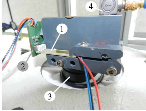
Figure 2. Experimental setup : (1) bender with a magnet and proof mass fixed at the end; (2) Hall sensor; (3) shaker; (4) accelerometer
