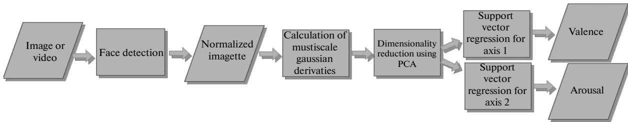
Fig. 7. Schematic of our approach.
