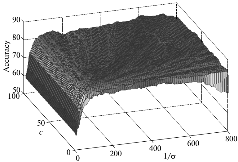
Fig. 3. Graph of Classification Accuracy vs. C-parameter and \sigma for Pleasure.
