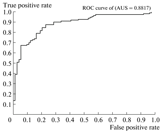
Fig. 9. ROC of the classifier for Arousal.
