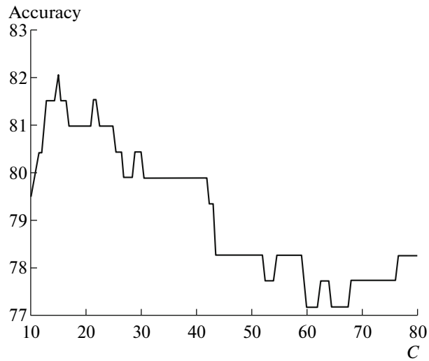
Fig. 6. Graph of Classification Accuracy vs. C-parameter at \sigma = 81 for Arousal.
