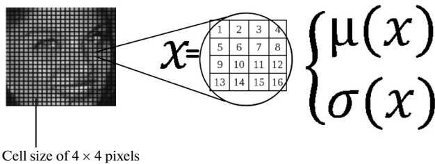
Fig. 2. The image divided into cells of 4 × 4 pixels.
