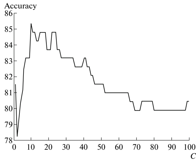
Fig. 4. Graph of Classification Accuracy vs. C-parameter at \sigma = 81 for Pleasure.
