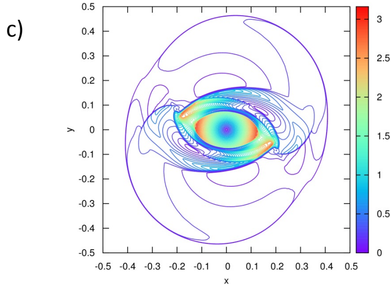
Figs. 10a, 10b, 10c and 10d show the density, gas pressure, Mach number and magnetic pressure for the MHD Rotor problem. The MuSIC Riemann solver with least square projection that was based on the one-dimensional HLLC Riemann solver was used.
