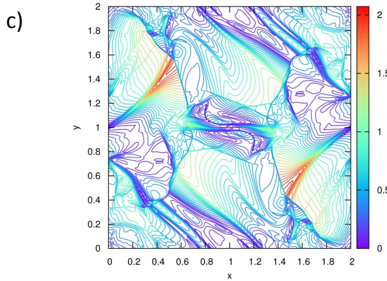
Figs. 11a, 11b, 11c and 11d show the density, gas pressure, Mach number and magnetic pressure for the MHD Orszag-Tang problem. The MuSIC Riemann solver with least square projection that was based on the one-dimensional HLLC Riemann solver was used.
