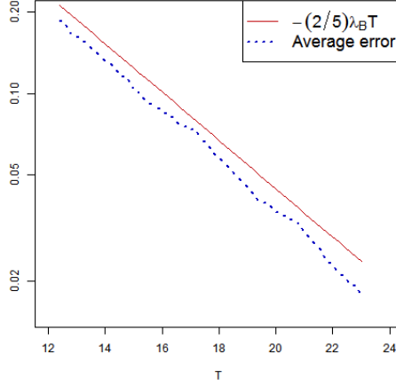
FIGURE 3. The log-average relative empirical error over M = 100 Monte-Carlo continuous trees vs. T (i.e. the log-rate) for x \rightsquigarrow B(x) reconstructed over \mathcal{D} = [0.25, 2.5] with x \rightsquigarrow \widehat{B}_T(x) (dashed blue line) compared to the expected log-rate (solid red line).
