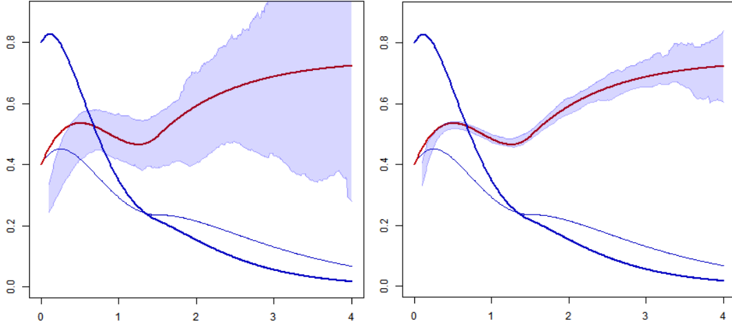
FIGURE 2. Reconstruction of B over \mathcal{D} = [0.1, 4] with 95%-level confidence bands constructed over M = 100 Monte-Carlo continuous trees. In bold red line: x \rightsquigarrow B(x) ; in bold blue line: f_{H_B} ; in blue line: f_B (on the same y -axis scale). Left: T = 15 . Right: T = 23 .
