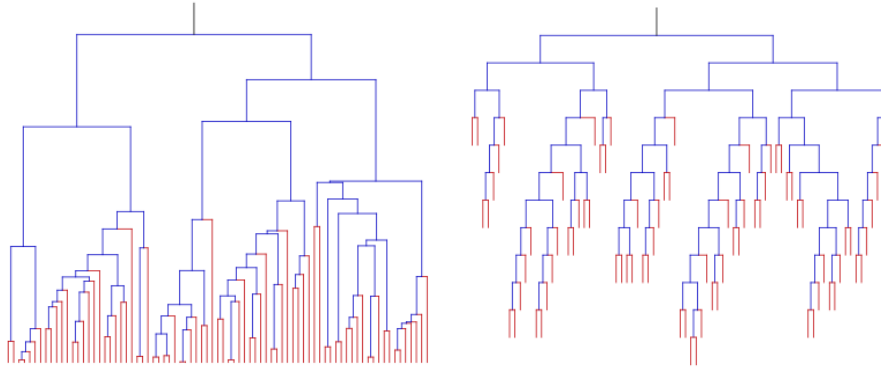
FIGURE 1. The effect of bias selection. Simulation of a binary ( p_2 = 1 so m = 2 ) age-dependent tree with B given in Section 4, up to time T = 8 ( |\mathcal{T}_T| = 145 ). Left: the size of each segment represents the lifetime of an individual. Individuals alive at time T are represented in red. Right: genealogical representation of the same realisation of the tree.
