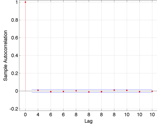
FIGURE 1. Sample autocorrelation of ordered (X_{u0}, u \in \mathbb{G}_{n-1}) for n = 15 . Note: due to the binary tree structure the lags are \{4, 6, 8, \dots\} . As expected, we observe a fast decorrelation.
