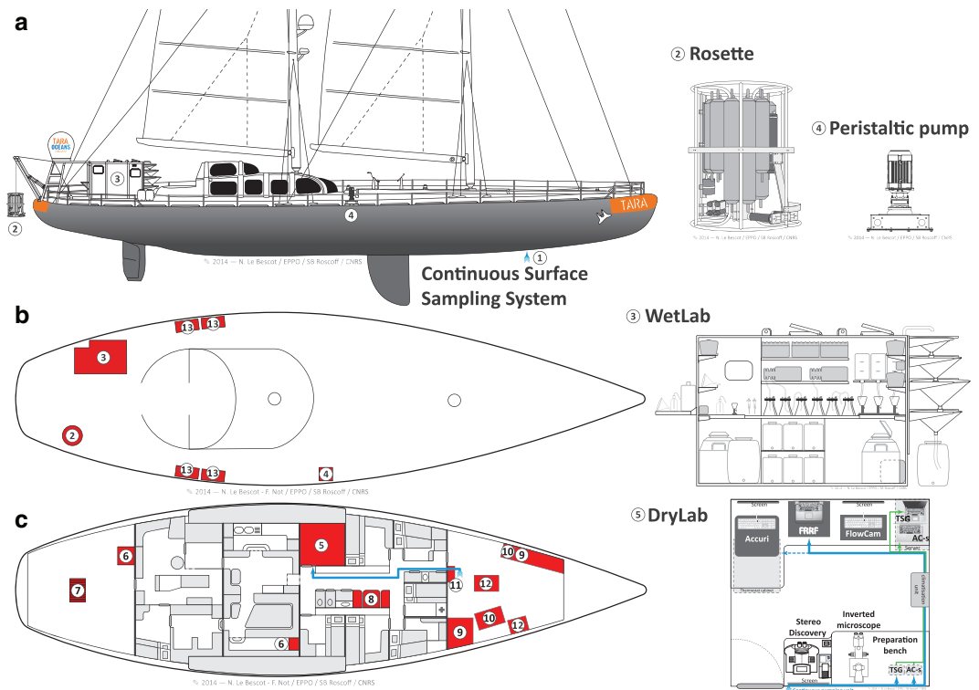
Figure 1. Sampling devices and working areas on-board SV Tara. Sampling devices and working areas on-board SV Tara are shown from the vessel's [a] side-view, [b] bird's-eye-view of the deck, and [c] inside-view. They consist of the [1] Continuous Surface Sampling System [CSSS]; [2] Rosette Vertical Sampling System [RVSS]; [3] wet lab and storage in liquid nitrogen; [4] High Volume Peristaltic pump [HVP-PUMP]; [5] dry lab; [6] oceanography engineers data acquisition and processing area; [7] winch; [8] video imaging area; [9] storage areas at room temperature; [10] storage areas at +4 °C and -20 °C; [11] MilliQ water system and AC-s system; [12] diving equipment, flowcytobot and ALPHA instruments; and [13] storage boxes. The flow of seawater from the continuous surface sampling system to the dry lab is shown in blue.
