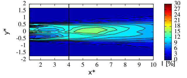
(a) Single turbine turbulence intensity map
