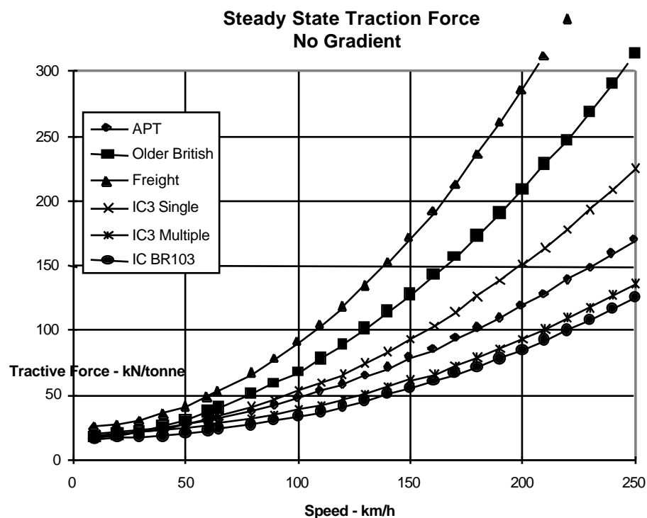
Figure 15: Traction force in kN/tonne for different types of railway trains as a function of train speed.
