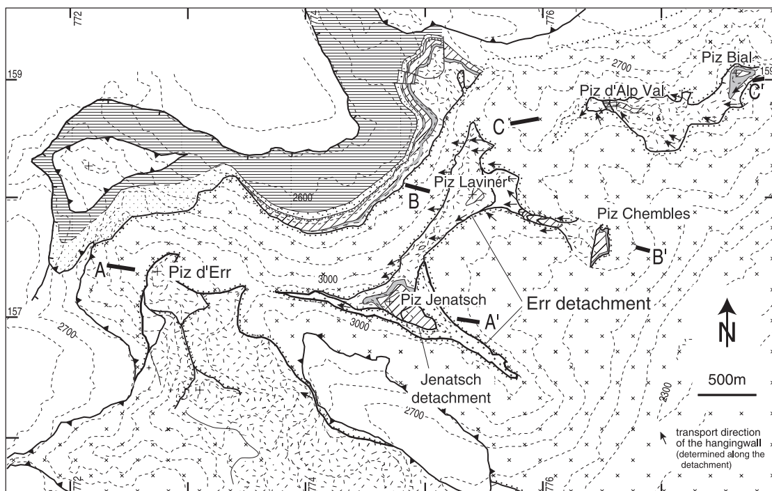
(a) Geological map of the Err region
