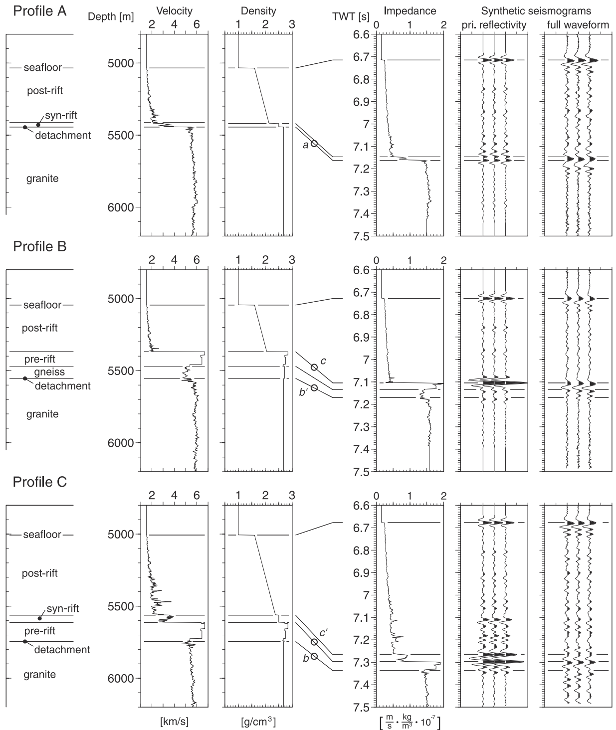
Figure 8. Seismic structure and response of crucial interfaces. The profiles and interface-labels correspond to those in Figures 6 and 7. The velocity and density structures are given as functions of depth, whereas the impedance profile is converted to two-way-travel time (TWT). The synthetic seismograms marked as “pri. reflectivity” are based on reflection coefficient sequences convolved with a Ricker wavelet with a center frequency of 35 Hz. The seismograms denoted as “full waveform” are extracted at corresponding locations from the time-migrated section shown in Figure 7b. See text for a discussion of the particular interfaces.
