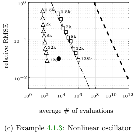
Figure 4: Relative root-mean-square error (RMSE) as a function of the average number of evaluations, over 100 independent runs, on Examples 4.1.1–4.1.3. For the subset simulation algorithm (squares) and for the BSS algorithm (triangles), the results are provided for several values of the sample size ( m \in \{500, 1000, 2000, \dots\} ). For the 2 SMART algorithm (filled circles), only one result is presented, corresponding to the default settings of the algorithm. The expected performance of plain Monte Carlo sampling is represented by a dashed line. The mixed line represents a simple approximation of the relative RMSE for the subset simulation algorithm: \frac{T_\alpha}{m} \frac{1-p_0}{p_0} , where T_\alpha = \lceil \frac{\log \alpha}{\log p_0} \rceil .
