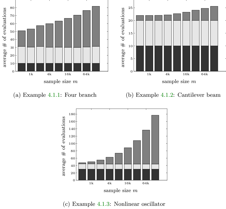
Figure 3: Average number of evaluations used by the BSS algorithm, over 100 independent runs, as a function of the sample size m on Examples 4.1.1–4.1.3. The total number of evaluations is split in three parts: the size n_0 of the initial design (dark gray), the number \sum_{t=1}^{T-1} N_t of evaluations in intermediate stages (light gray) and the number of evaluations N_T in the final stage (middle gray).
