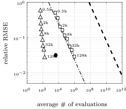
(c) Example 4.1.3: Nonlinear oscillator
