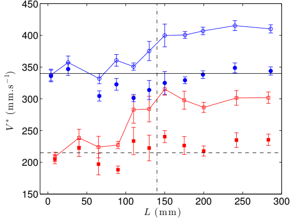
Figure 7: Evolution of the threshold velocity V_d^* for capture as a function of the fiber length L for R = 0.76 mm and \nu = 1 \times 10^{-6} \text{ m}^2 \cdot \text{s}^{-1} (red hollow squares) and \nu = 5 \times 10^{-6} \text{ m}^2 \cdot \text{s}^{-1} (blue hollow circles). The threshold velocities are rescaled by the relative speed of the fiber given by equation (12) (filled symbol). The horizontal lines indicate the threshold velocities for L = 0 mm and the vertical dashed-dotted line corresponds to L = 140 mm.
