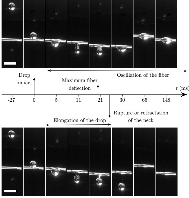
Figure 2: Image sequences of a drop of radius R = 0.76 mm impacting a fiber ( L = 14 cm, 2a = 400 \mu m) at different velocities V_d (side view). For V_d = 370 mm.s ^{-1} the drop is captured by the fiber (top images) whereas for V_d = 390 mm.s ^{-1} the drop is released (bottom images). Scale bar: 2 mm.
