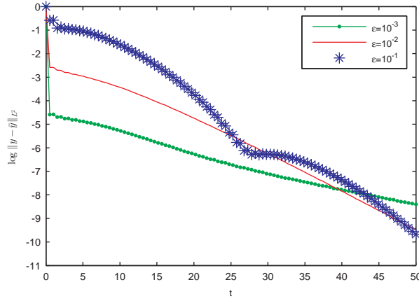
Figure 1: Time evolutions of \log \|y(\cdot, t) - \bar{y}(\cdot, t)\|_{L^2}^2 for different values of \epsilon with initial conditions belonging to H^2 .
