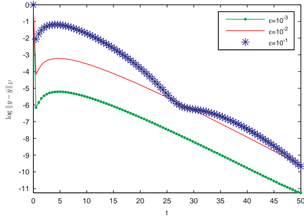
Figure 2: Time evolutions of \log \|y(\cdot, t) - \bar{y}(\cdot, t)\|_{L^2}^2 for different values of \epsilon with the particular initial condition z^0 = \frac{G_{21}}{1-G_{22}}y^0(1) .
