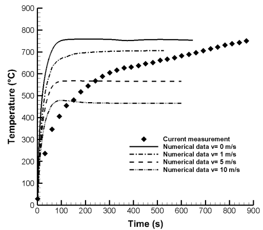
Figure 9: TC 1 temperature evolution in the cooling configuration
