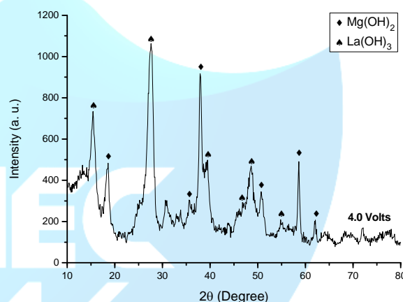
Fig. 3. X-ray diffraction pattern of the sample
