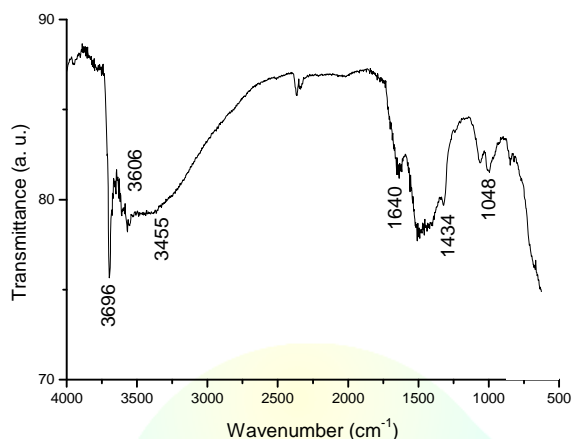
Fig. 4. FTIR transmittance spectrum of the as-prepared powder
