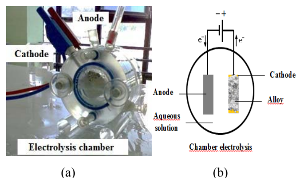
Fig. 1. Illustrations of the electrodeposition experimental setup. (a) Photograph and (b) schematic overview.
