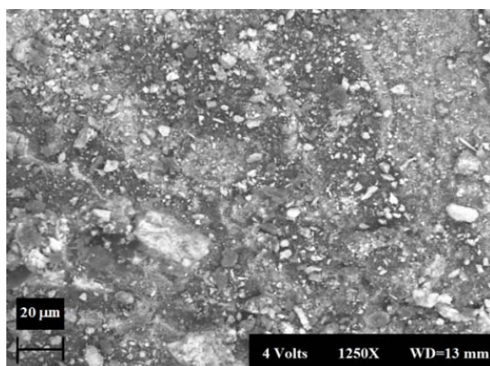
Fig. 2. SEM image of the as-deposited powder
